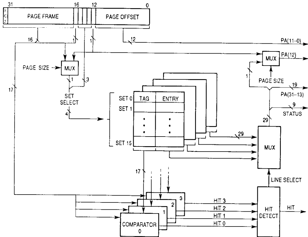
Figure 3-20. ATC Organization
