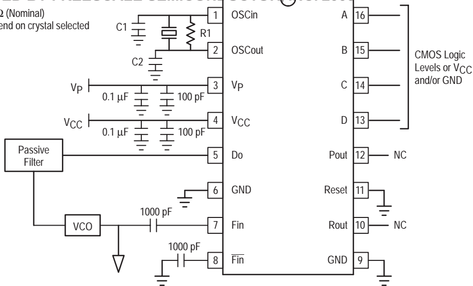
Figure 2. Typical Applications Example
