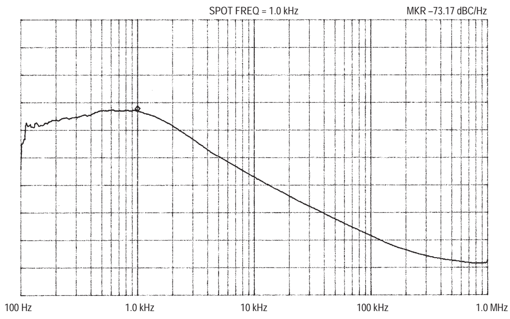
Figure 17. Typical Phase Noise Plot, 240MHz (Low Noise 10 MHz Reference Input)
