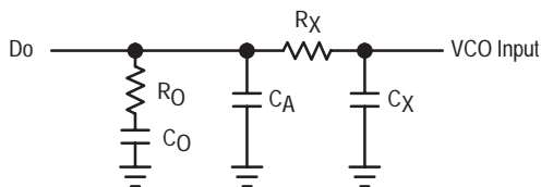
Figure 3. Typical Passive Loop Filter Topology
