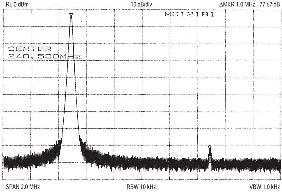
Figure 16. VCO Output Spectrum (P=30, 8.0 MHz ECLIPTEK Crystal)
