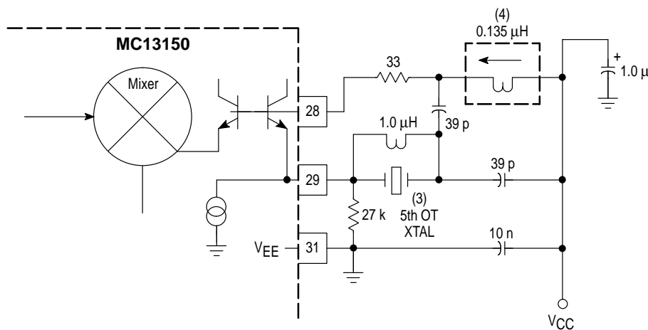
Figure 16. MC13150FTB Overtone Oscillator f_{RF} = 83.16 \text{ MHz} ; f_{LO} = 83.616 \text{ MHz} 5th Overtone Crystal Oscillator
