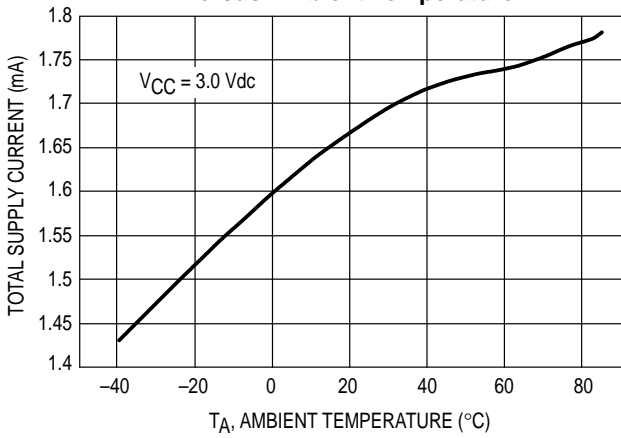
ARCHIVED BY FREESCALE SEMICONDUCTOR, INC. 2005 Figure 21. Total Supply Current versus Ambient Temperature
