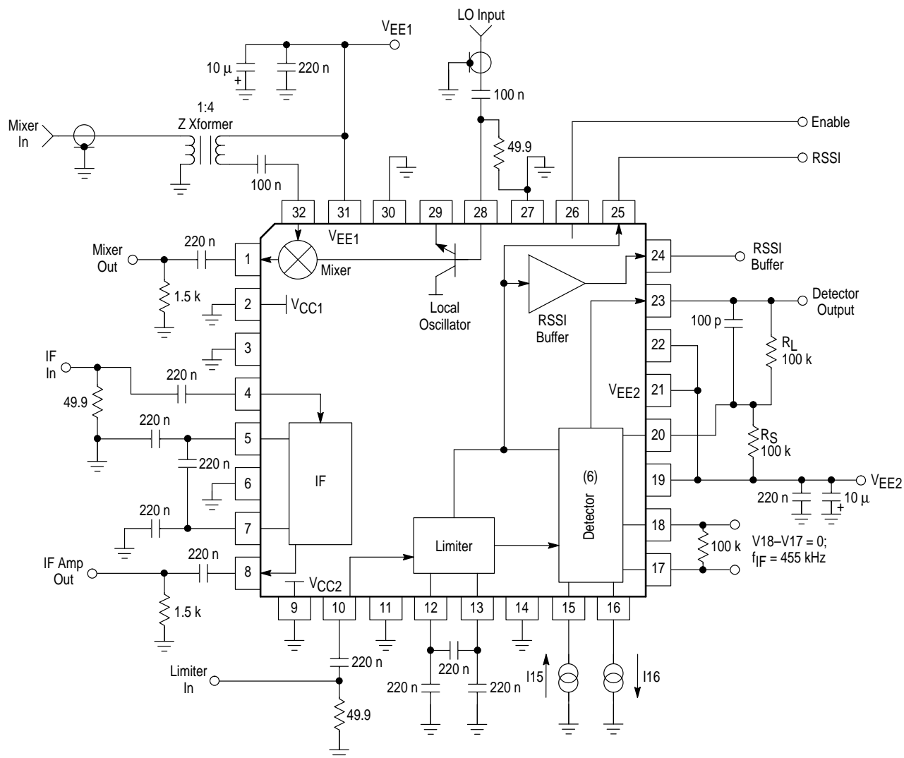
Figure 1. Test Circuit
