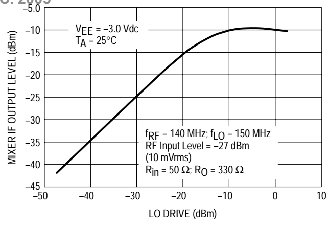
Figure 10. Mixer IF Output Level versus Local Oscillator Input Level
