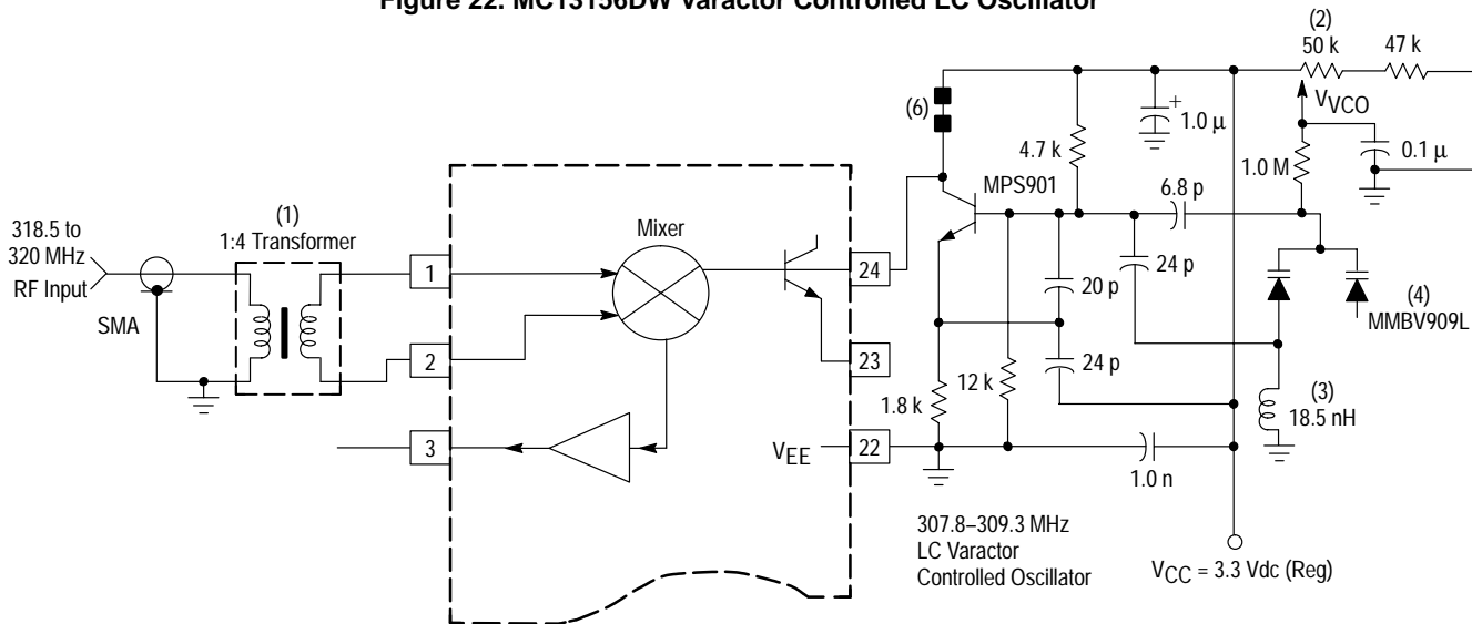
Figure 22. MC13156DW Varactor Controlled LC Oscillator
