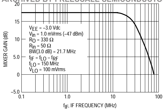
Figure 9. Mixer Gain versus IF Frequency
