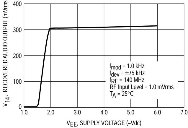
Figure 13. Recovered Audio Output Voltage versus Supply Voltage
