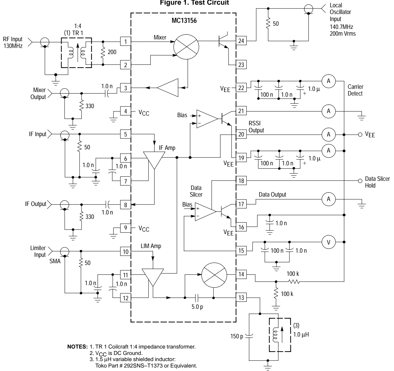
Figure 1. Test Circuit
