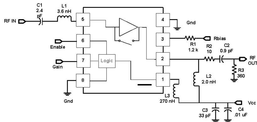
Figure 10. 2400 MHz Application Schematic
