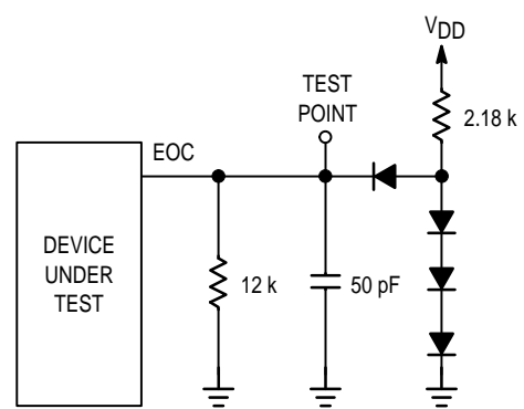
Figure 8. Test Circuit
