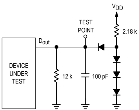
Figure 7. Test Circuit
