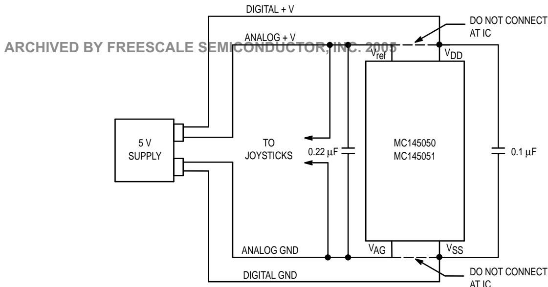
Figure 16. Alternate Configuration Using the Digital Supply for the Reference Voltage
