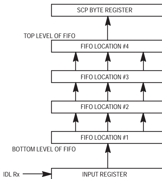
Figure 12-2. Receive FIFOs
