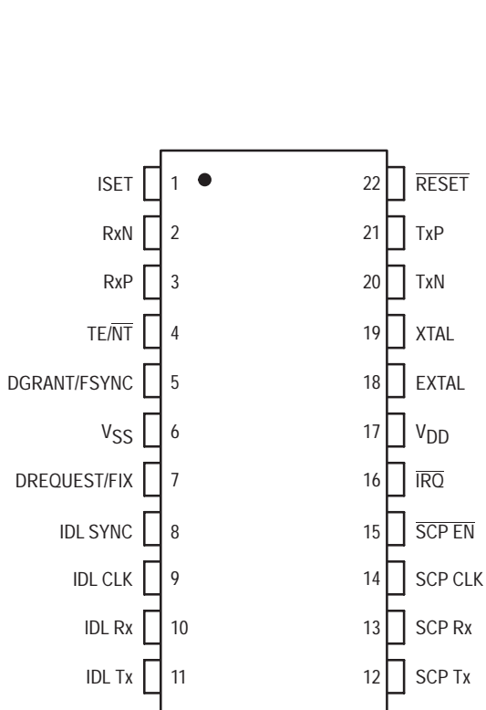
Figure 6-1. MC145474 Pin Assignment
