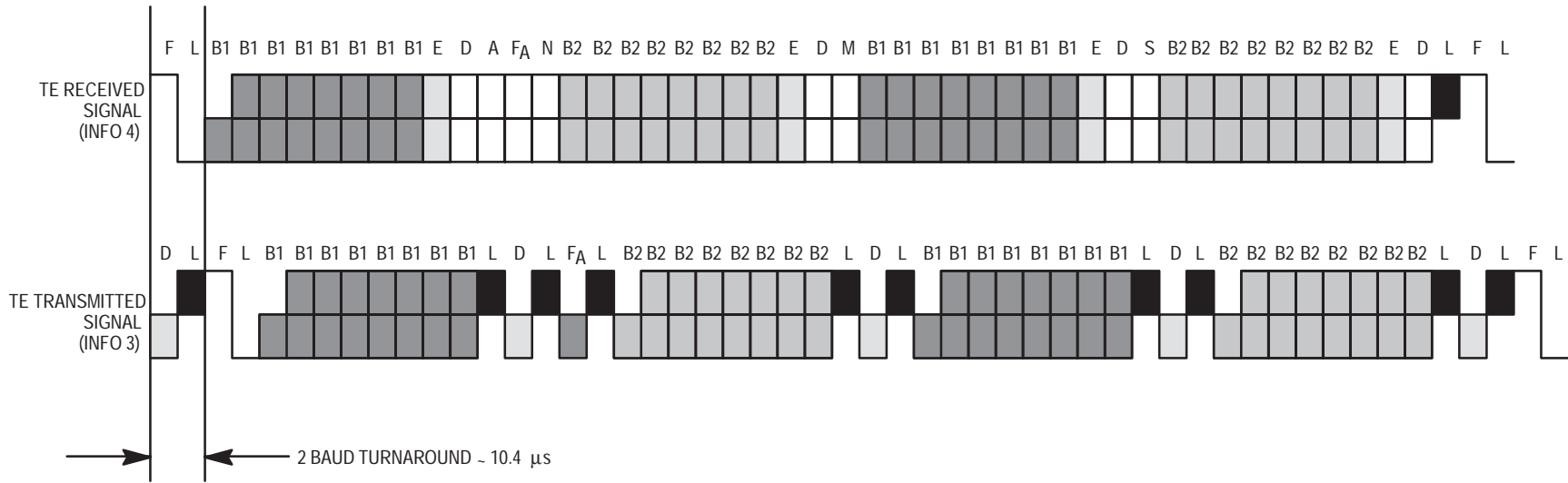
Figure 4-3. Two Baud Turnaround in TE
