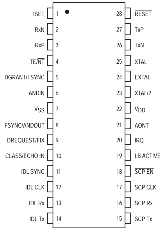
Figure 16-2. MC145475 Pin Assignment
