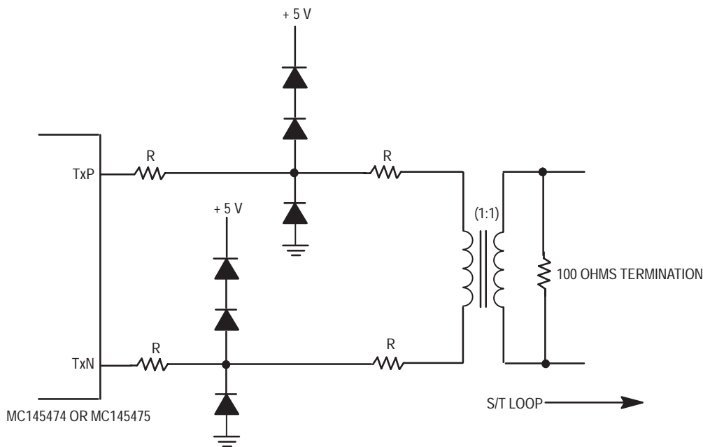
Figure 14-1. Transmit Line Interface Circuit
