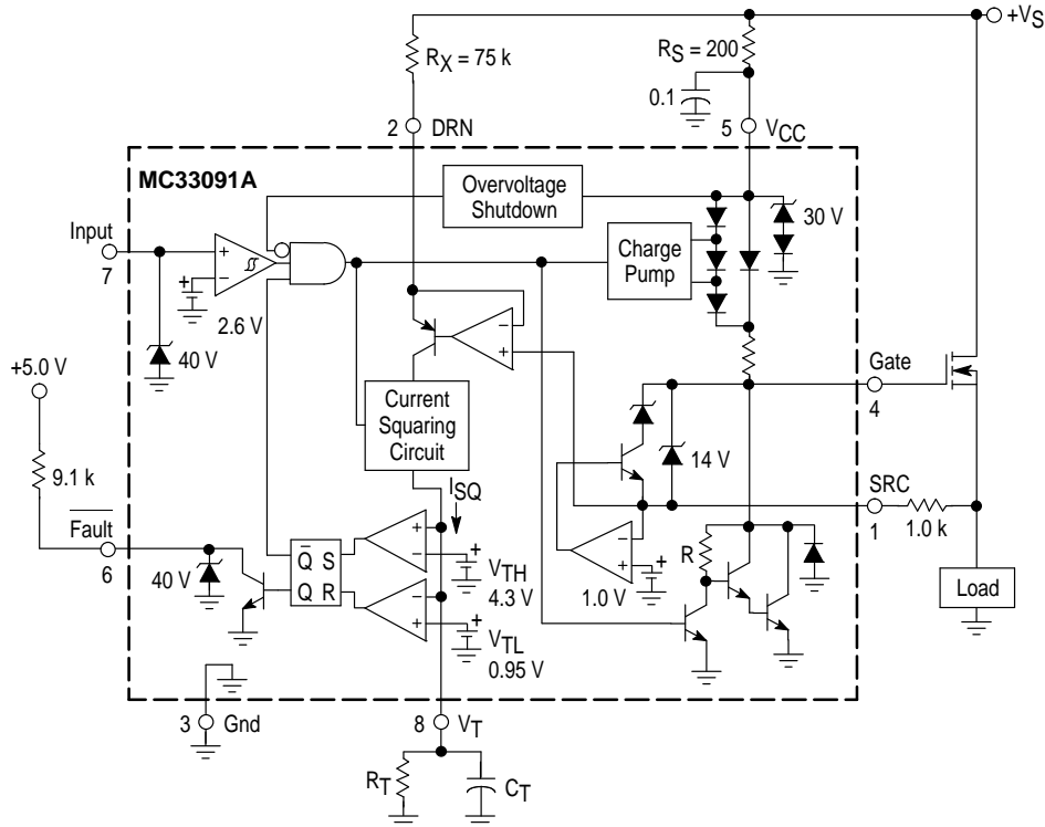
Figure 1. Typical Application
