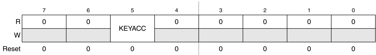
Figure 15-4. ROM Configuration Register (RCNFG)
