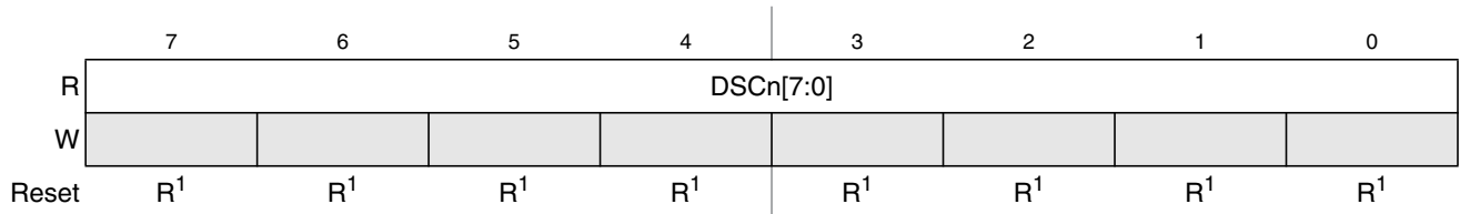
Figure 15-5. ROM Device SC Number Register (RDSC0–RDSC2)
