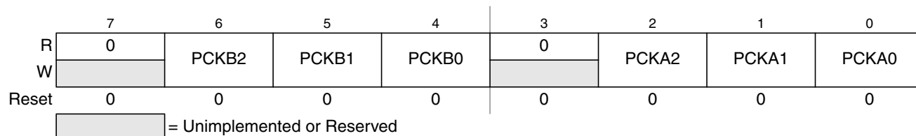
Figure 14-6. PWM Prescale Clock Select Register (PWMPRCLK)
