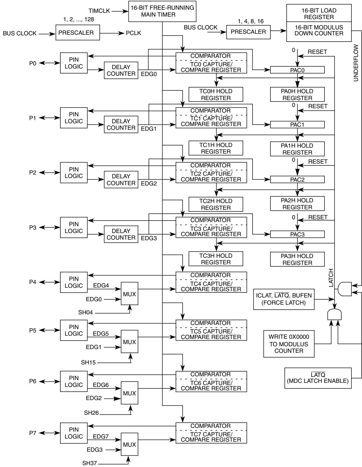
Figure 10-37. Detailed Timer Block Diagram in Latch Mode
