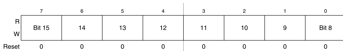
Figure 7-6. Breakpoint First Address High Byte Register (BKP0H)
