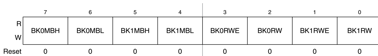
Figure 7-4. Breakpoint Control Register 1 (BKPCT1)
