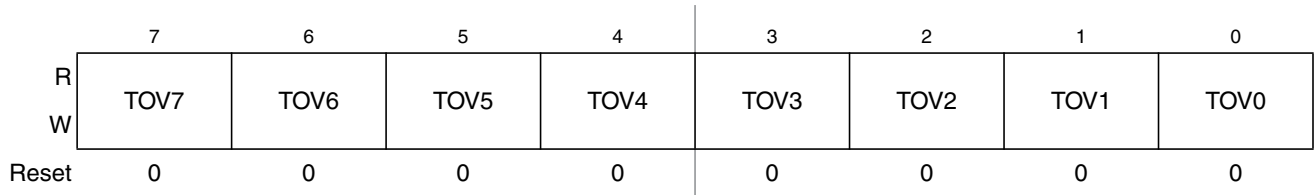
Figure 10-9. Timer Toggle On Overflow Register 1 (TTOV)
