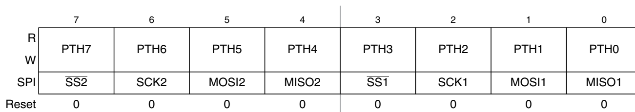
Figure 2-32. Port H I/O Register (PTH)
