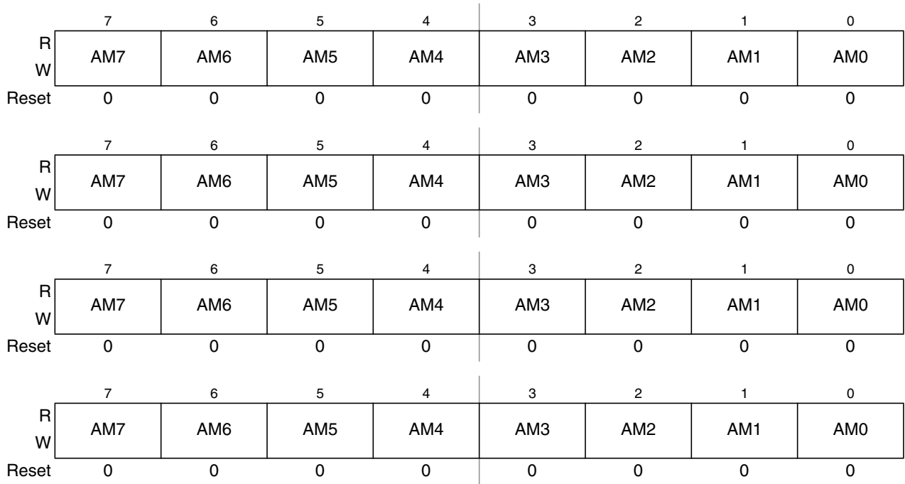
Figure 12-22. MSCAN Identifier Mask Registers (Second Bank) — CANIDMR4–CANIDMR7
