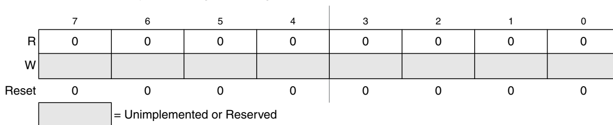
Figure 4-18. Reserved Register
