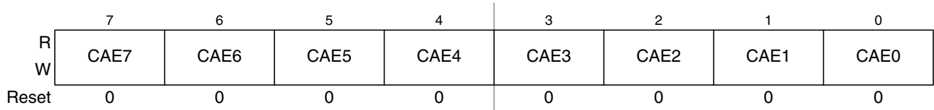
Figure 14-7. PWM Center Align Enable Register (PWMCAE)
