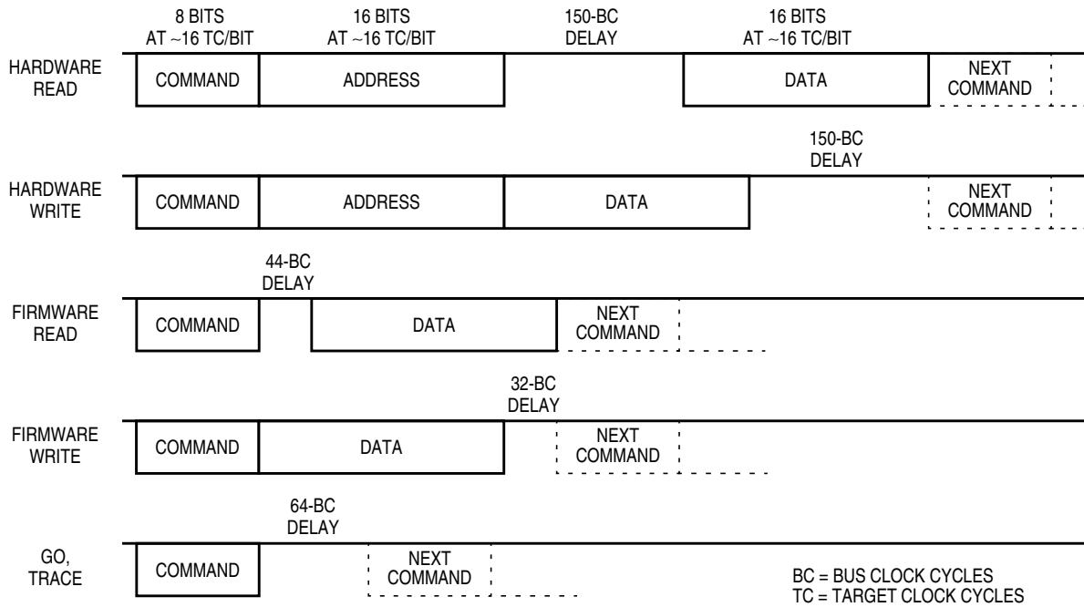
Figure 6-6. BDM Command Structure
