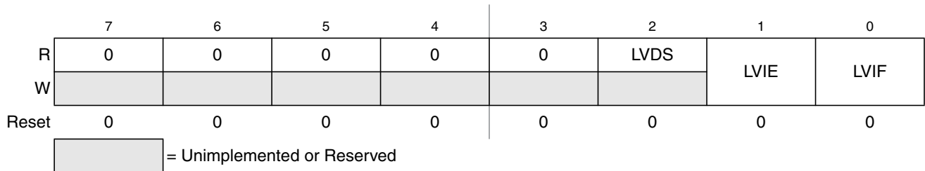
Figure 18-2. VREG3V3 — Control Register (VREGCTRL)
