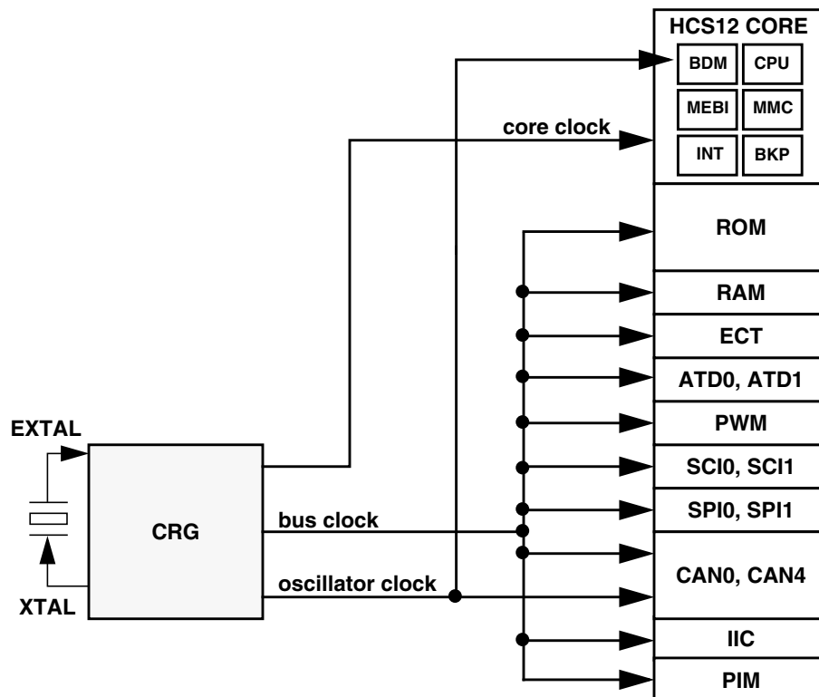
Figure 1-10. Clock Connections
