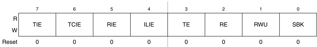
Figure 16-5. SCI Control Register 2 (SCICR2)
