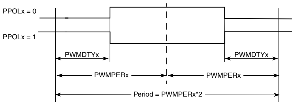
Figure 14-22. PWM Center Aligned Output Waveform
