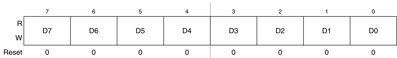
Figure 11-8. IIC Bus Data I/O Register (IBDR)
