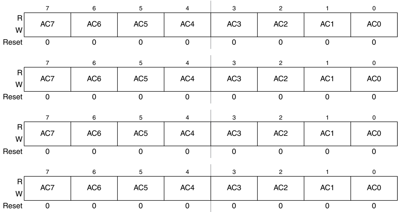
Figure 12-20. MSCAN Identifier Acceptance Registers (Second Bank) — CANIDAR4–CANIDAR7
