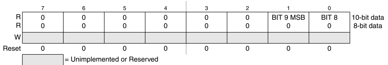
Figure 8-17. Right Justified, ATD Conversion Result Register, High Byte (ATDDRxH)
