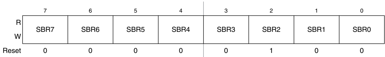
Figure 16-3. SCI Baud Rate Registers (SCIBDH and SCIBDL)
