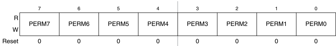
Figure 2-20. Port M Pull Device Enable Register (PERM)
