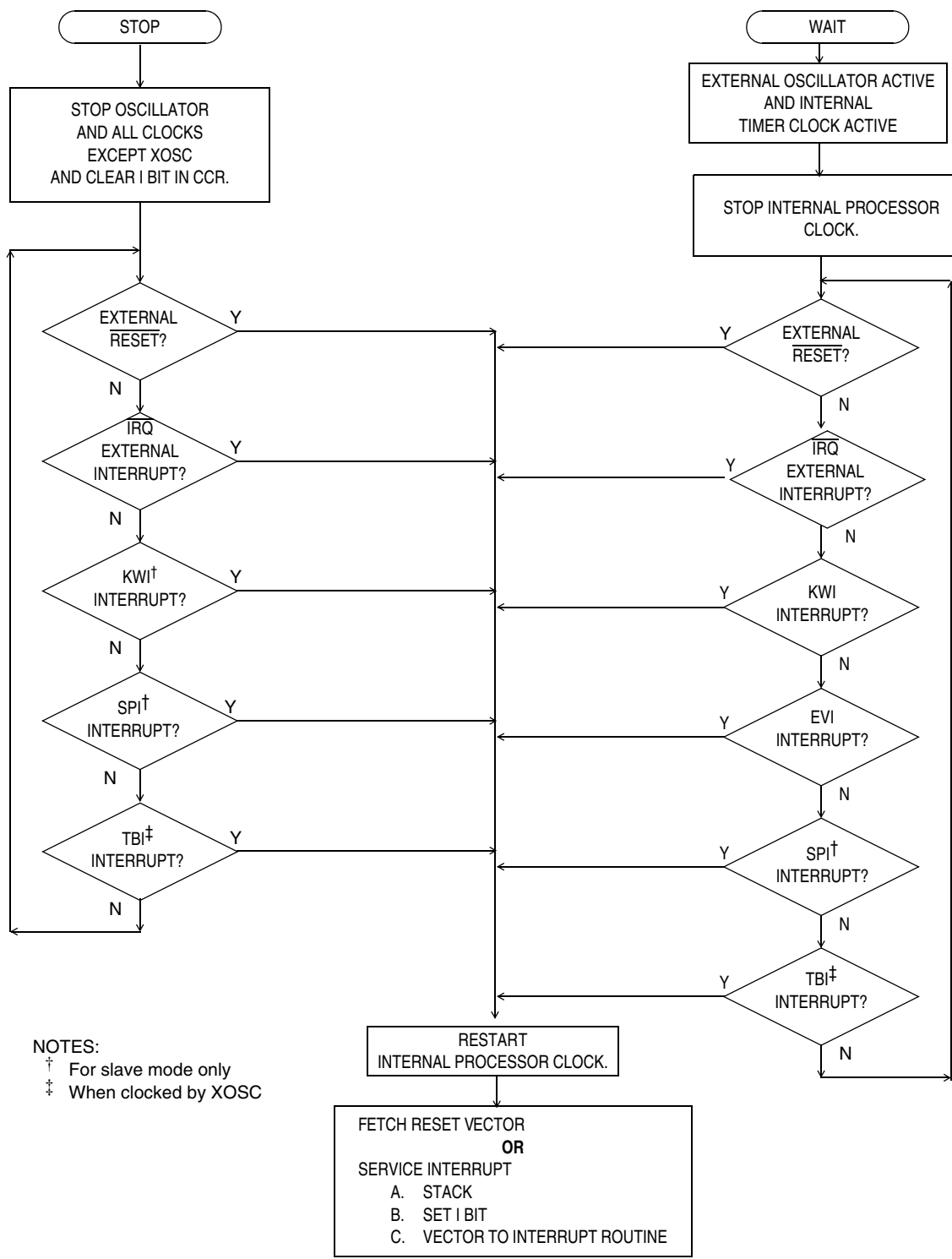
Figure 3-1. Stop/Wait Flowcharts
