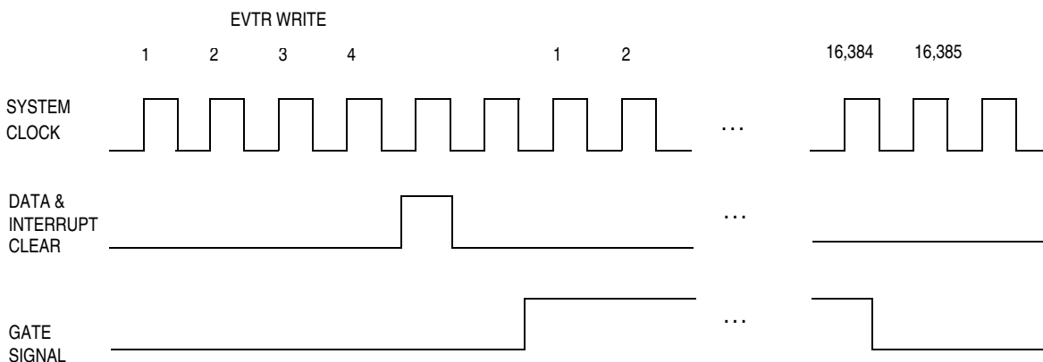
Figure 13-5. Event Counter Gate Signal Timing Example
