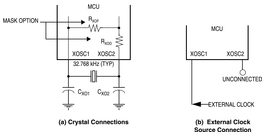
Figure 1-5. Oscillator Connections
