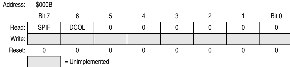
Figure 10-3. SPI Status Register (SPSR)
