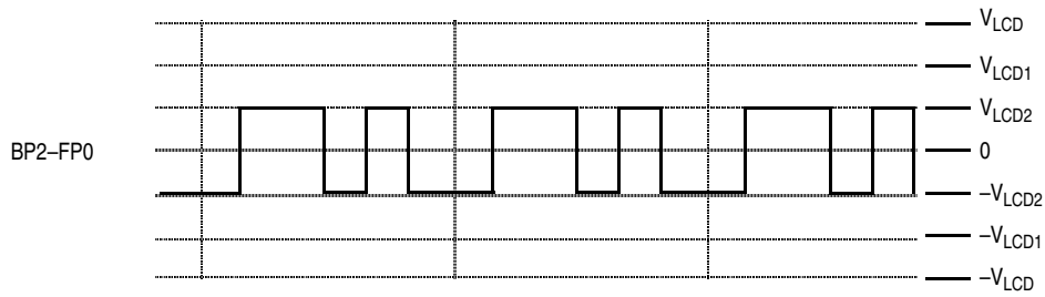
Figure 11-12. E Segment Electric Potential Waveform
