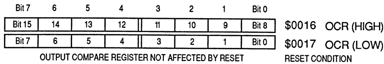
Figure 6-8. Output Compare Register (OCR)
