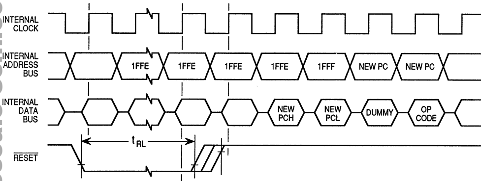
Figure 8-9. Power-On Reset Timing
