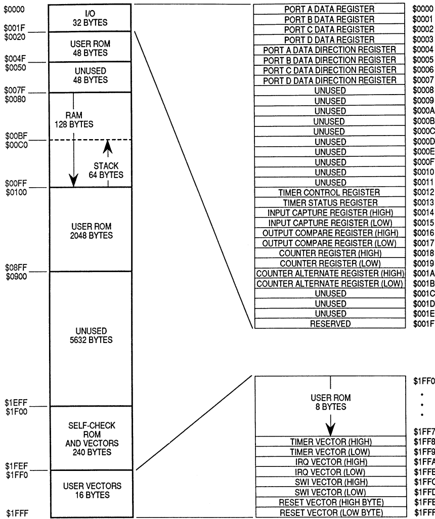
Figure 5-1. MC68HC05P1 Memory Map
