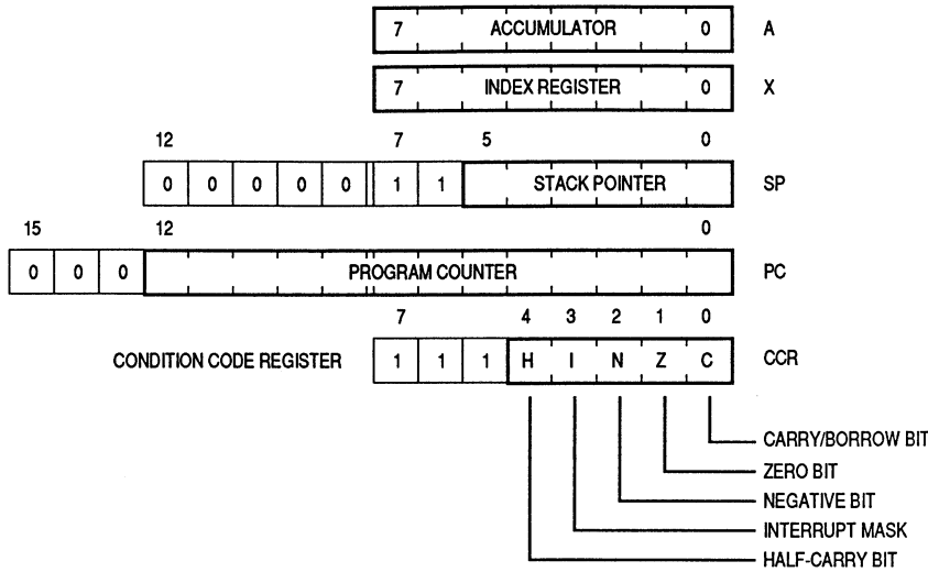
Figure 3-2. Programming Model
