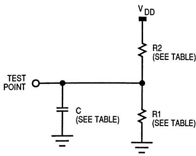
Figure 8-1. Test Load
