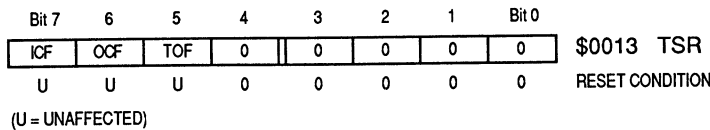
Figure 6-9. Timer Status Register (TSR)
