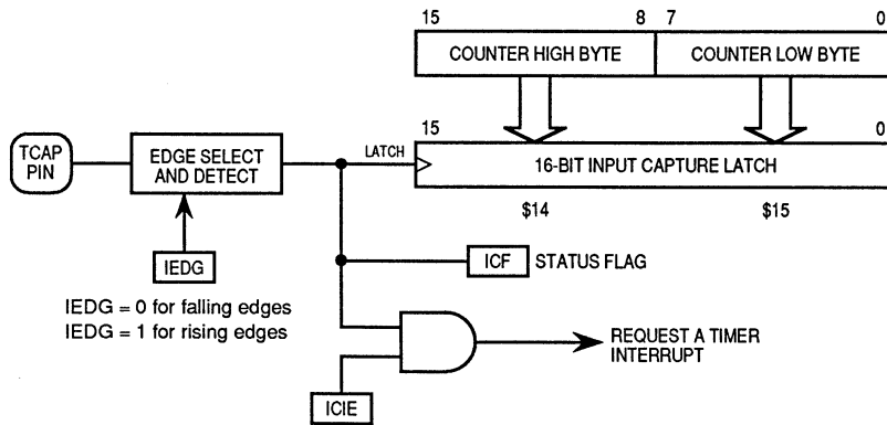
Figure 6-5. Input Capture Operation
