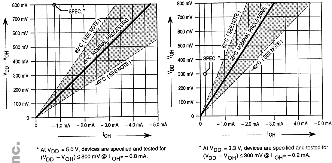
Figure 8-2. Typical High-Side Driver Characteristics
