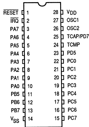
Figure 2-1. Pin Assignments
