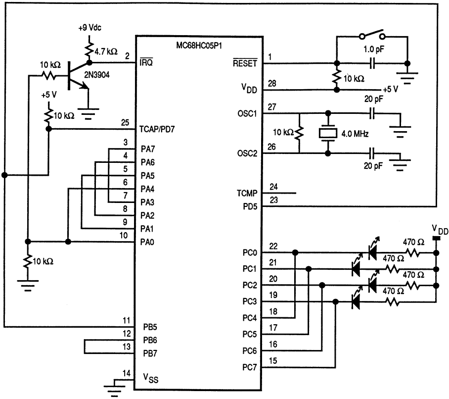
Figure 7-1. Self-Check Circuit
