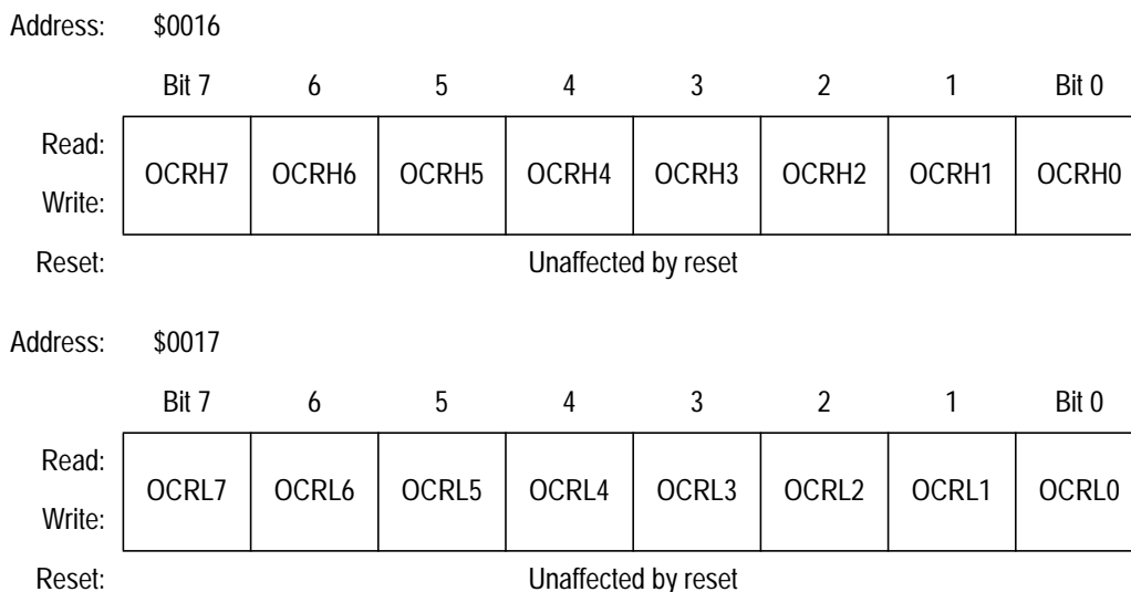
Figure 8-6. Output Compare Registers (OCRH/OCRL)
