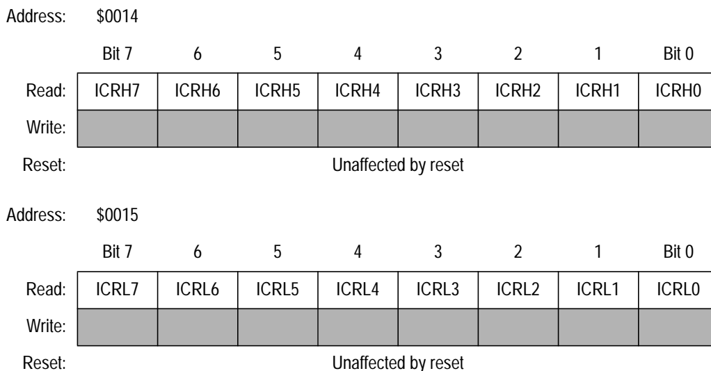
Figure 8-8. Input Capture Registers (ICRH/ICRL)
