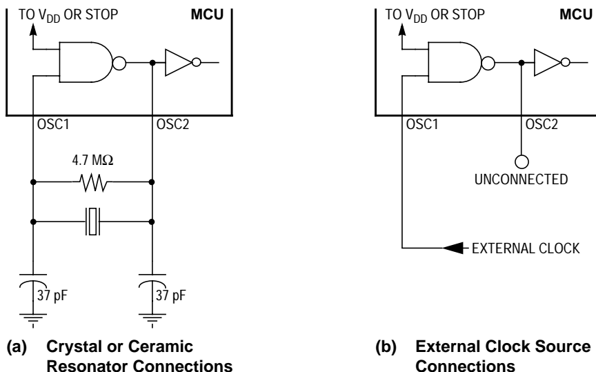
Figure 1-3. Oscillator Connections
