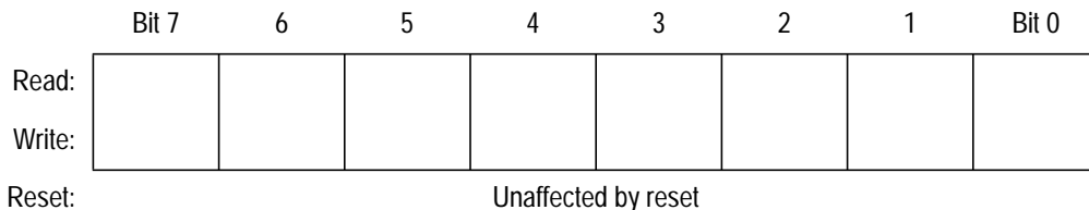
Figure 3-2. Accumulator (A)
