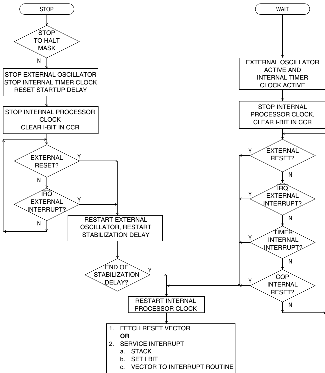
Figure 6-1. STOP/WAIT Flowchart
