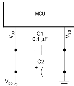
Figure 3. Bypassing Recommendation
