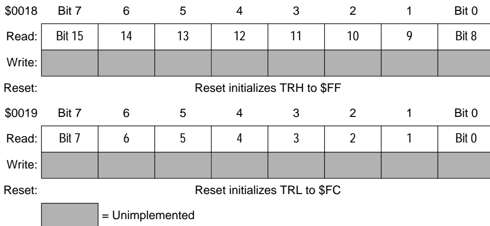
Figure 53. Timer Registers (TRH and TRL)
