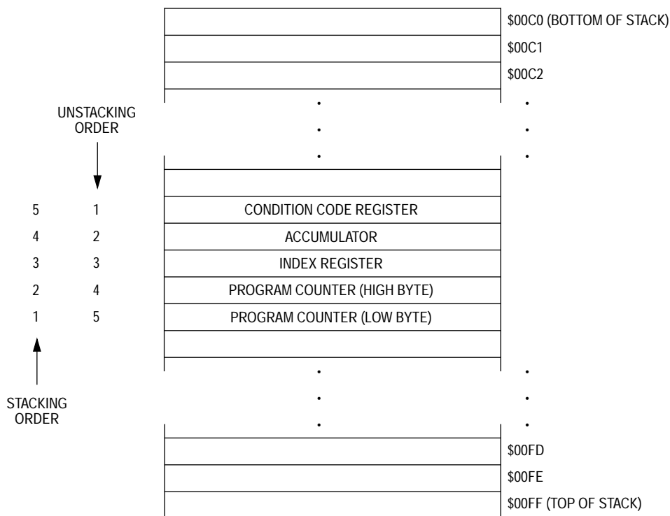
Figure 22. Interrupt Stacking Order
