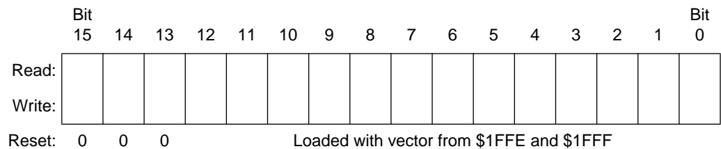
Figure 15. Program Counter (PC)
