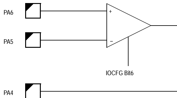
Figure 7-4 Operational Amplifier
