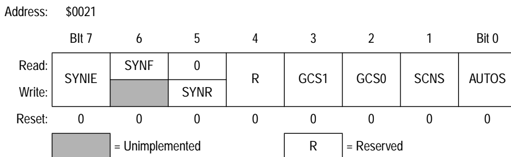
Figure 15-13. Scan Status and Control Register (SSCR)
