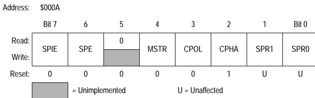
Figure 10-4. SPI Control Register (SPCR)
