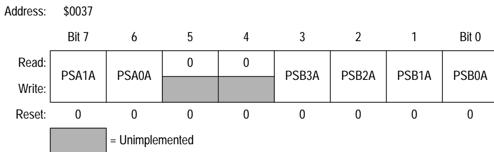
Figure 11-5. PWMA Control Register (PWMA)
