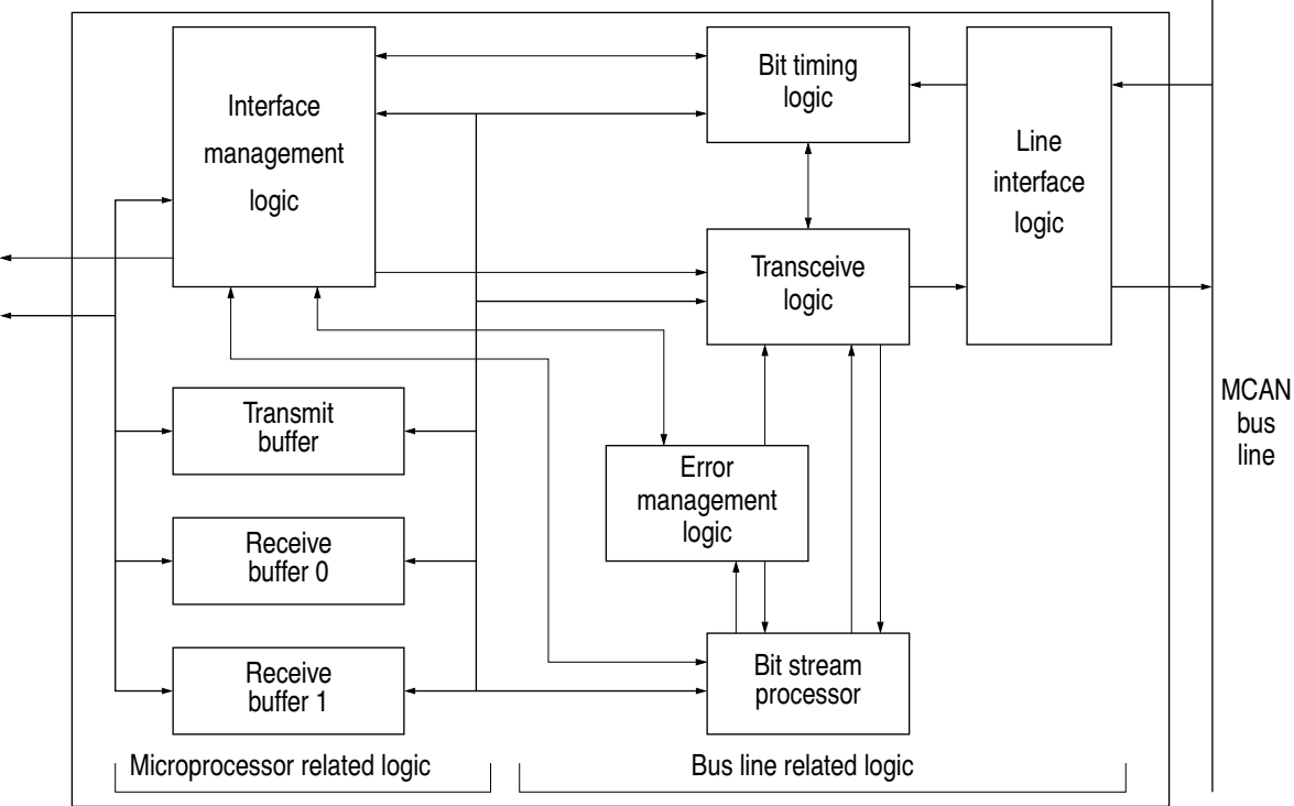
Figure 1. MCAN block diagram
