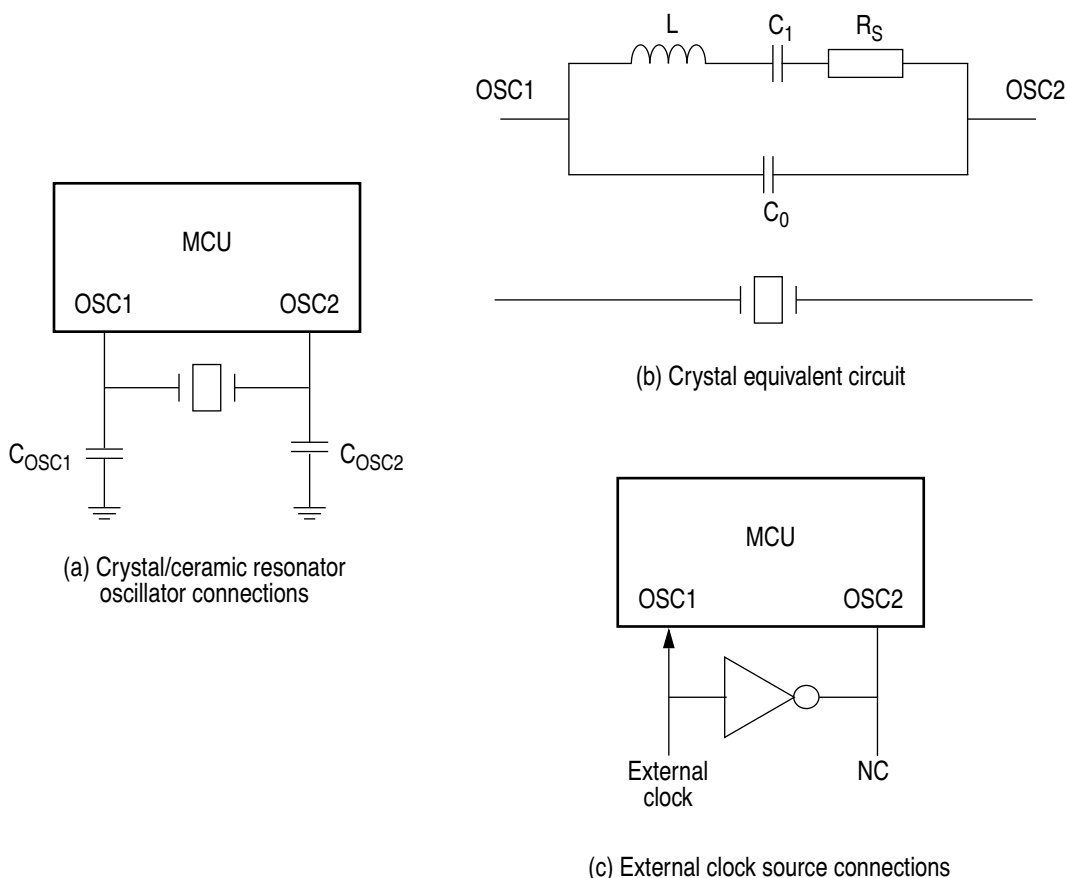
Figure 8. Oscillator connections
