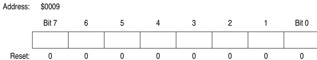
Figure 3. Core Timer Counter Register (CTCR)
