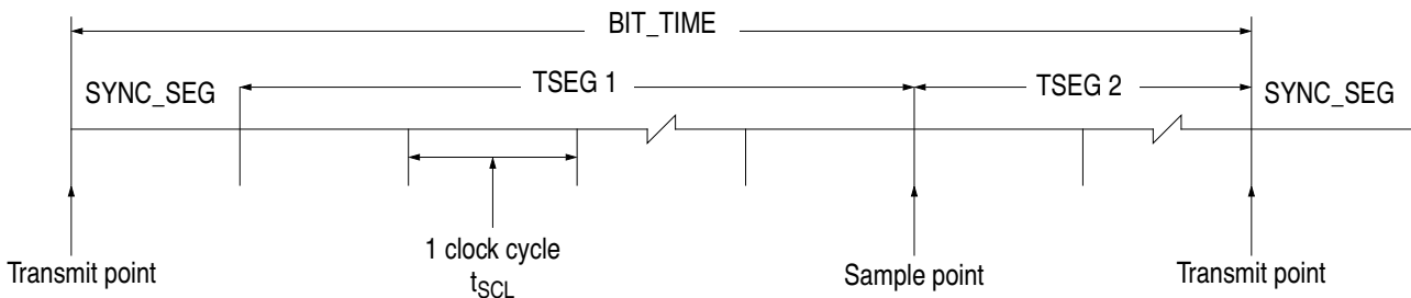
Figure 13. Segments within the bit time
