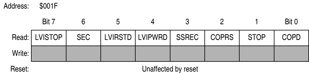
Figure 20-2. Mask Option Register A (MORA)
