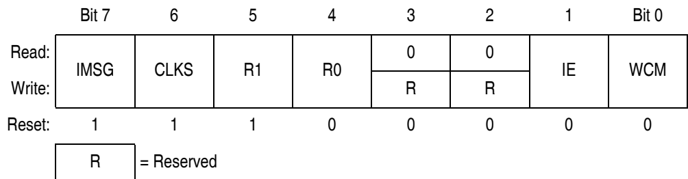
Figure 20-16. BDLC Control Register 1 (BCR1)
