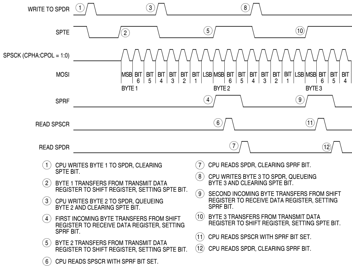
Figure 18-10. SPDR/SPTC CPU Interrupt Timing
