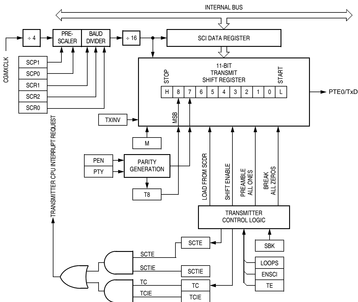
Figure 17-3. SCI Transmitter
