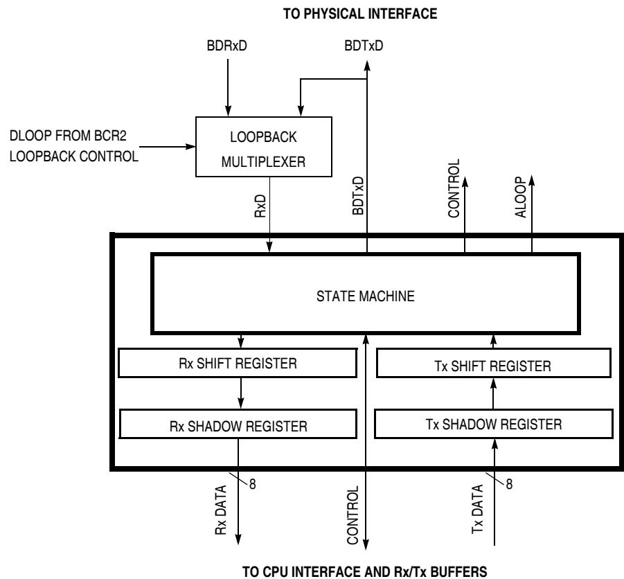
Figure 20-13. BDLIC Protocol Handler Outline
