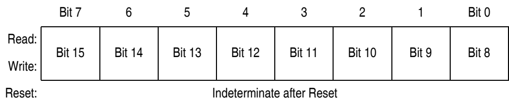
Figure 16-8. TIM Channel Registers (TCH0H/L–TCH3H/L) (Sheet 1 of 3)
