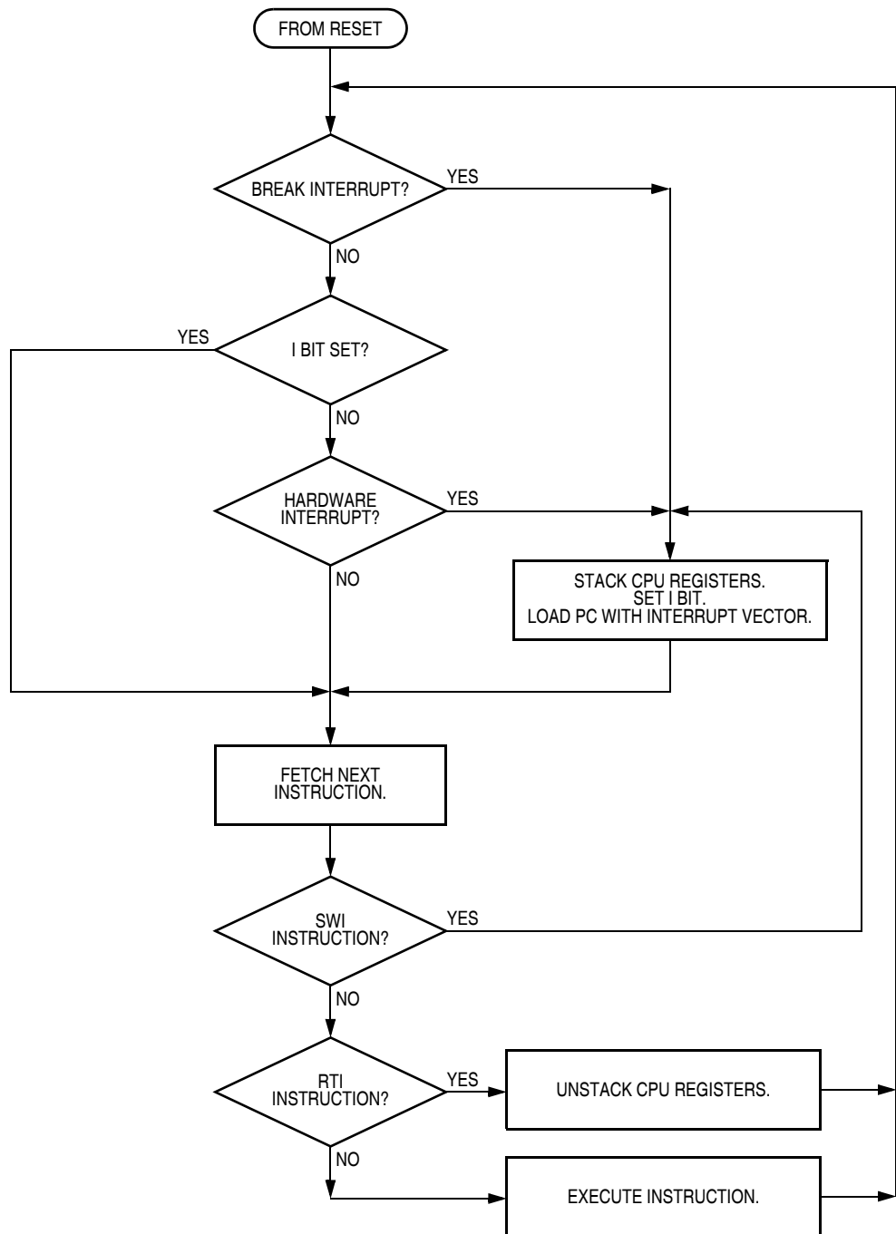
Figure 9-8. Interrupt Processing
