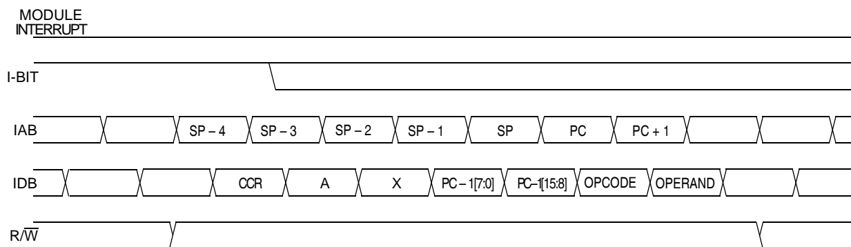
Figure 8-8. Interrupt Recovery
