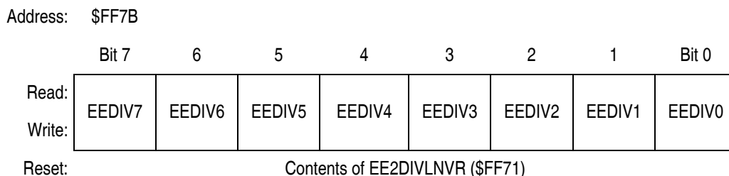
Figure 6-6. EE2DIV Divider Low Register (EE2DIVL)
