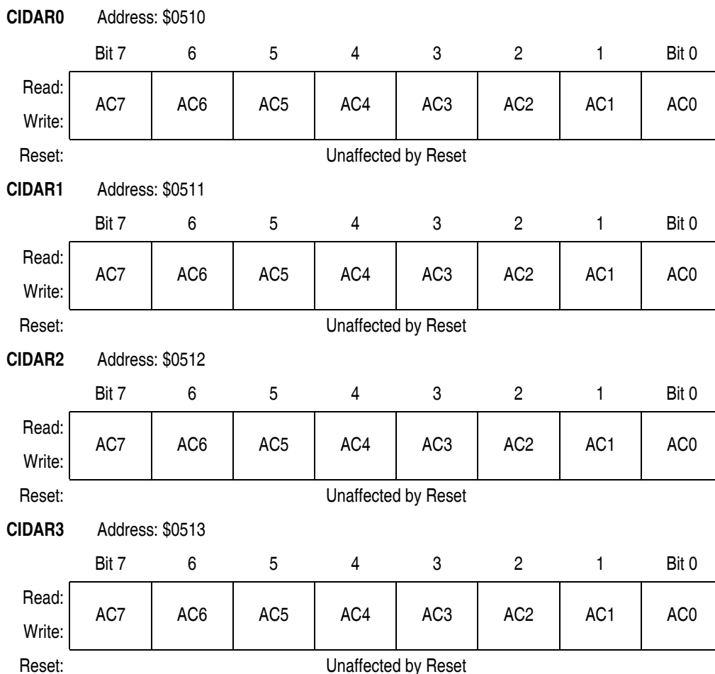
Figure 21-26. Identifier Acceptance Registers (CIDAR0–CIDAR3)
