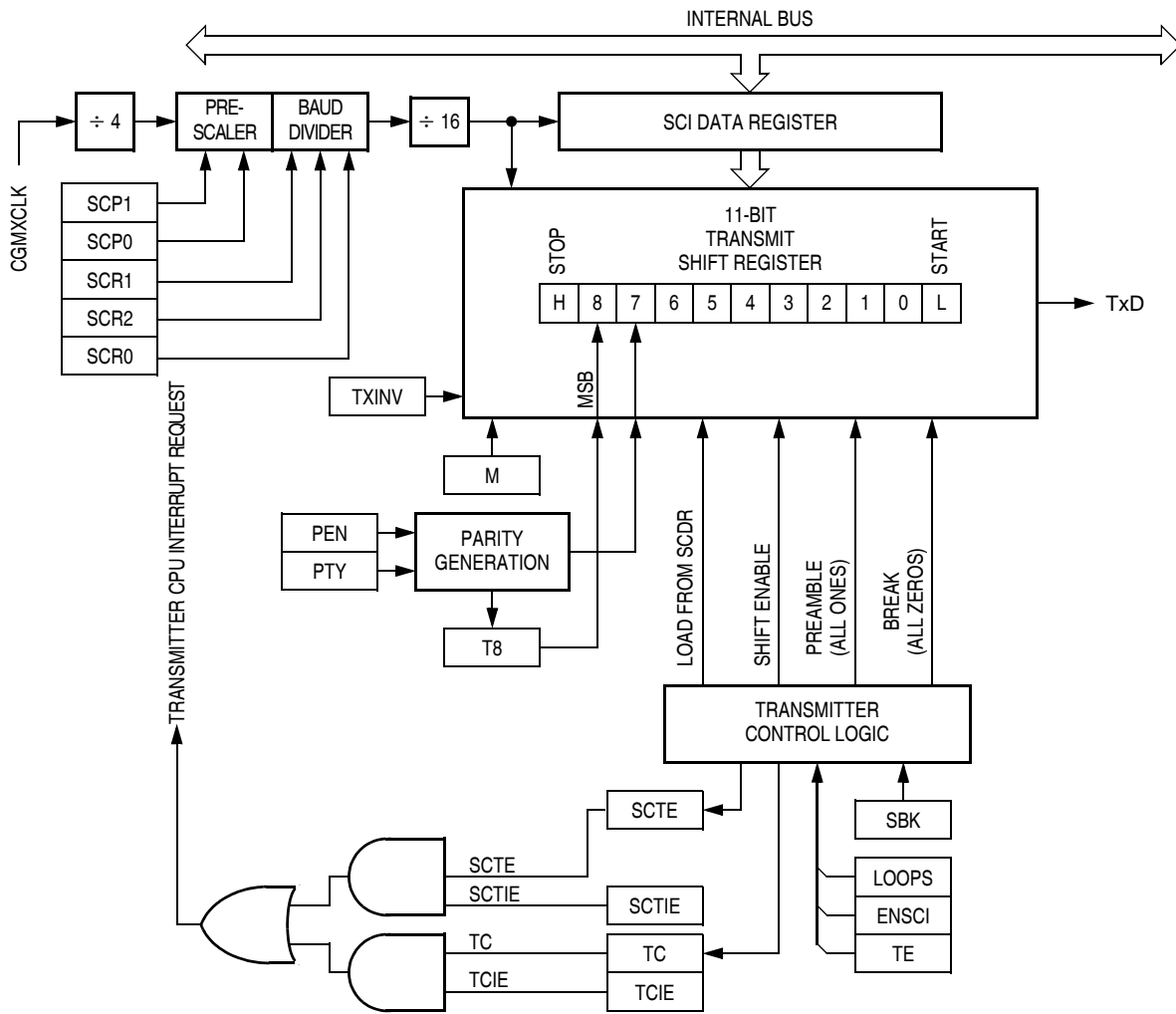
Figure 16-4. SCI Transmitter
