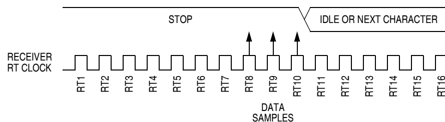
Figure 14-9. Fast Data
