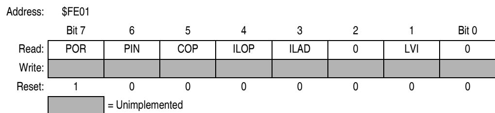
Figure 15-21. SIM Reset Status Register (SRSR)
