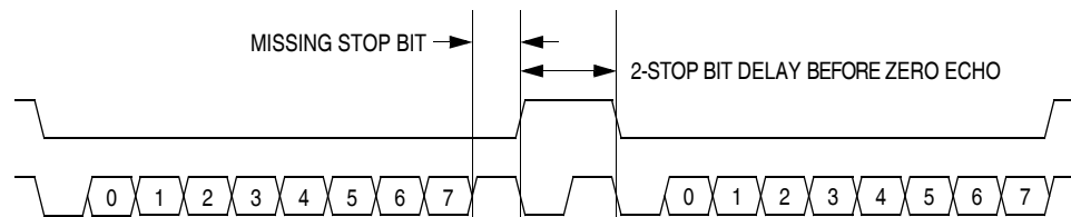
Figure 19-11. Break Transaction
