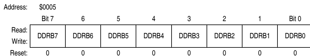
Figure 12-7. Data Direction Register B (DDRB)
