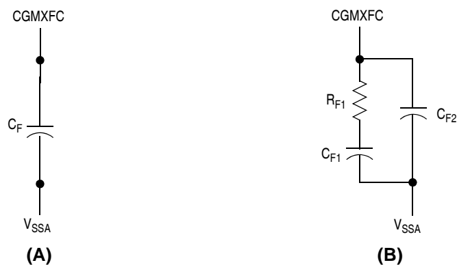
Figure 4-11. PLL Filter
