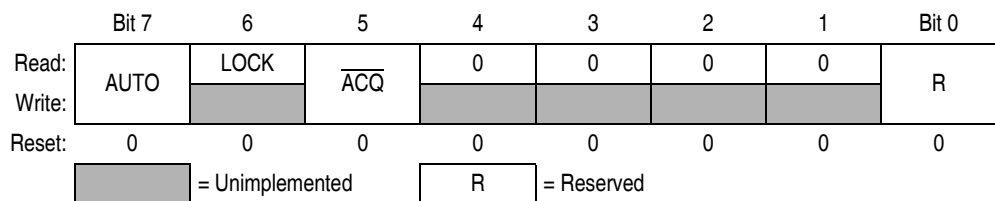
Figure 4-6. PLL Bandwidth Control Register (PBWC)
