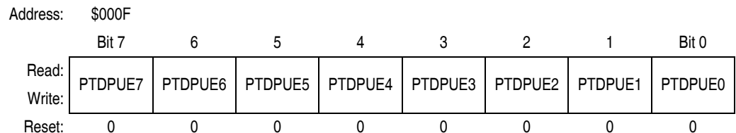
Figure 12-16. Port D Input Pullup Enable Register (PTDPUE)
