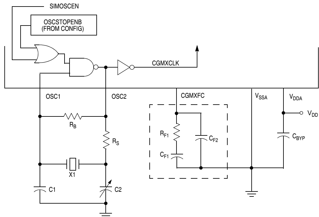
Figure 4-3. CGM External Connections
