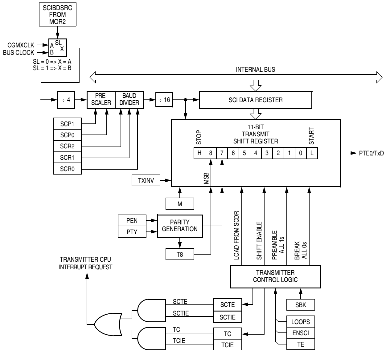
Figure 14-5. SCI Transmitter
