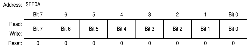
Figure 19-5. Break Address Register Low (BRKL)
