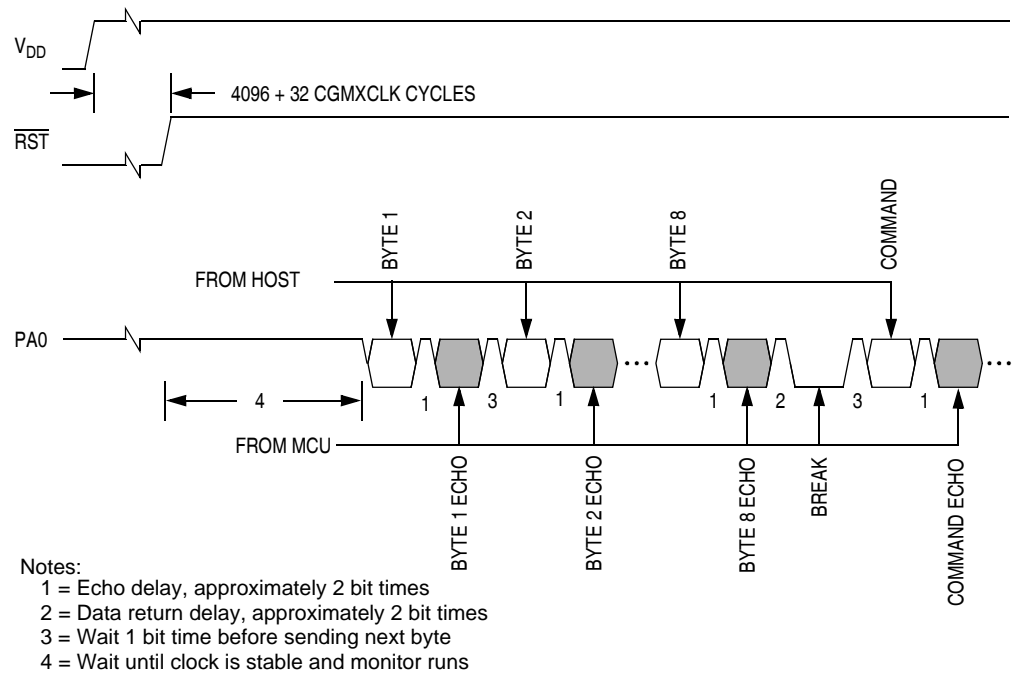
Figure 19-15. Monitor Mode Entry Timing
