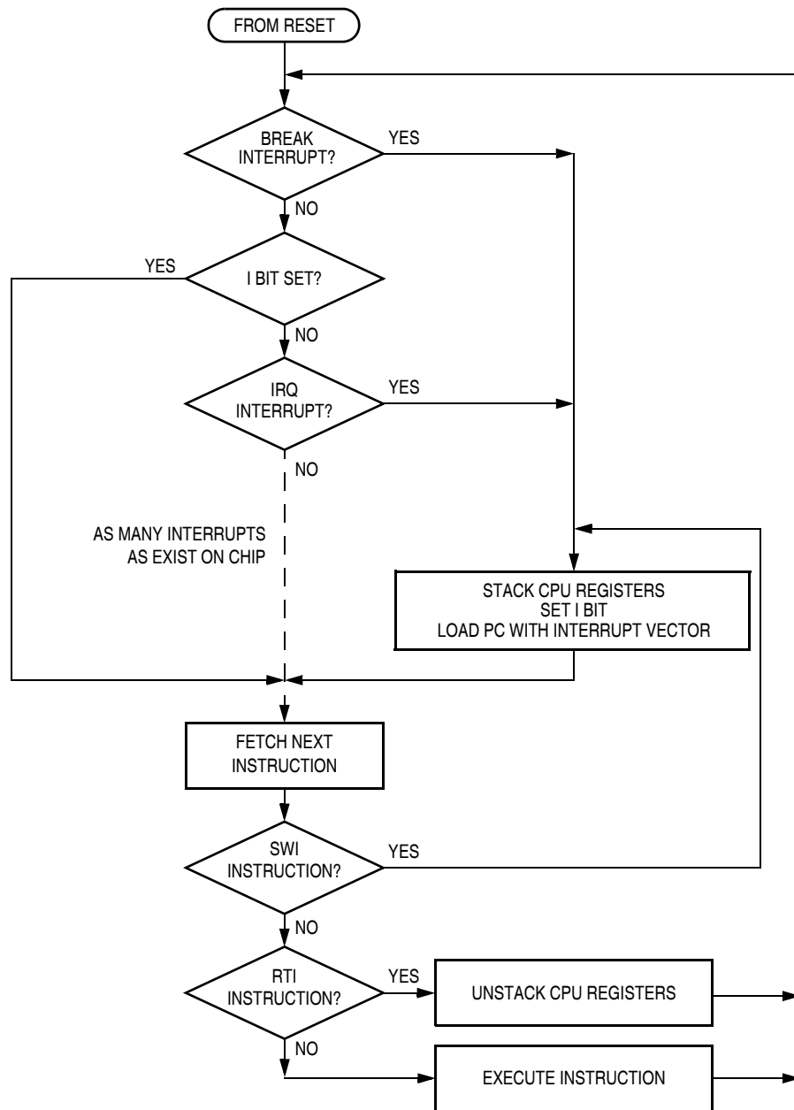
Figure 15-10. Interrupt Processing
