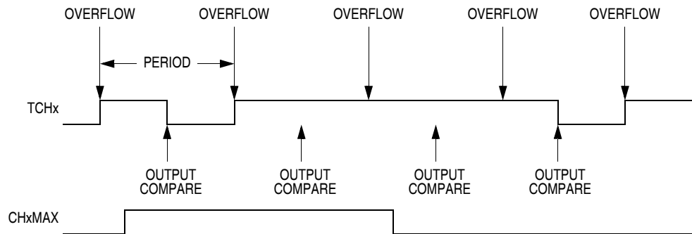
Figure 18-12. CHxMAX Latency
