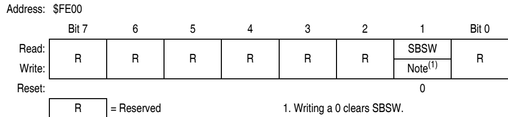
Figure 19-6. Break Status Register (SBSR)
