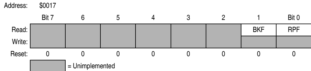
Figure 14-15. SCI Status Register 2 (SCS2)
