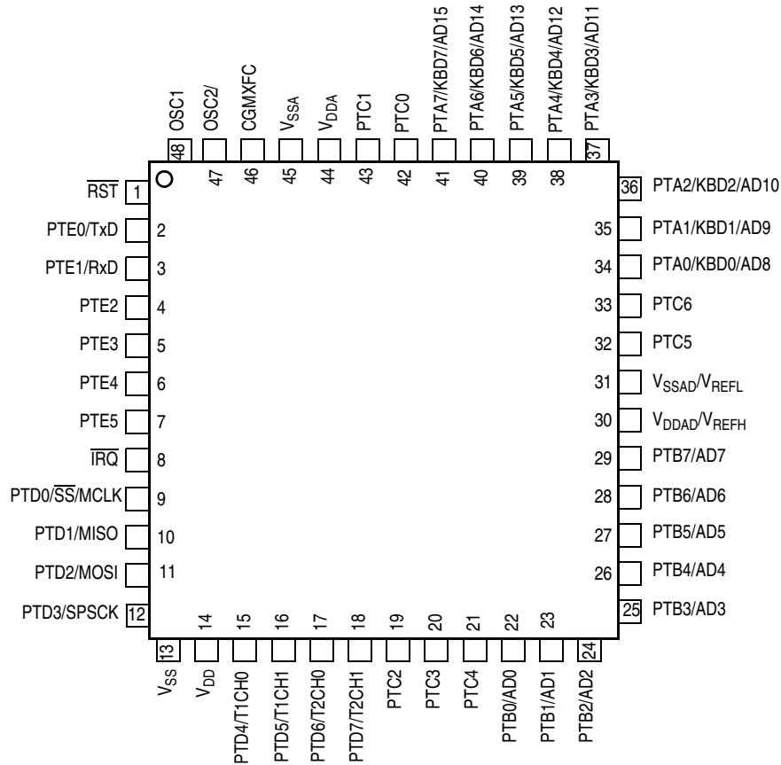
Figure 1-4. 48-Pin LQFP Pin Assignments
