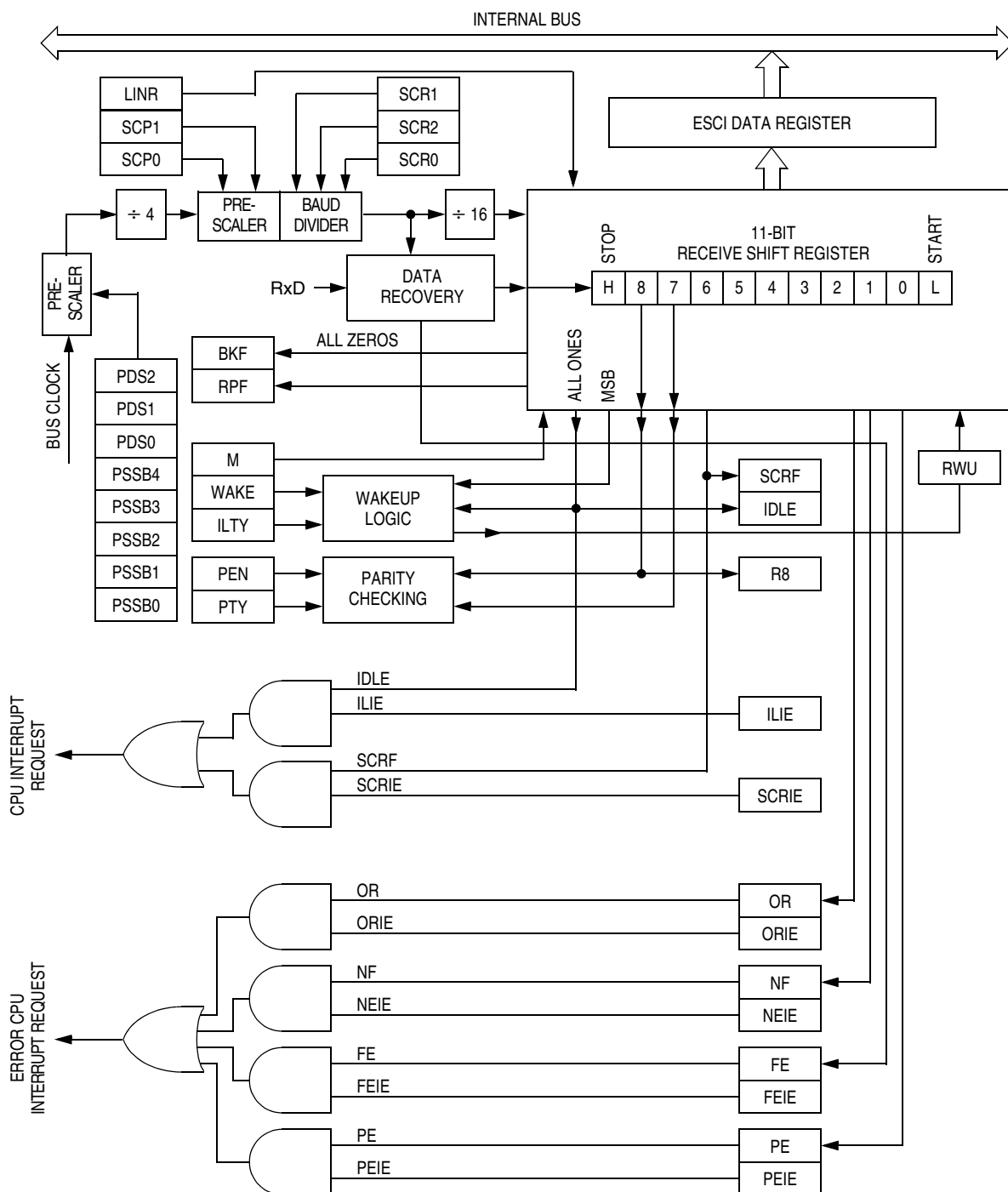
Figure 13-6. ESCI Receiver Block Diagram
