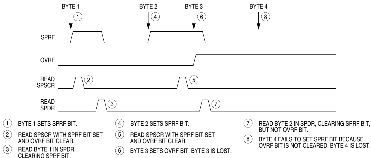
Figure 15-10. Missed Read of Overflow Condition
