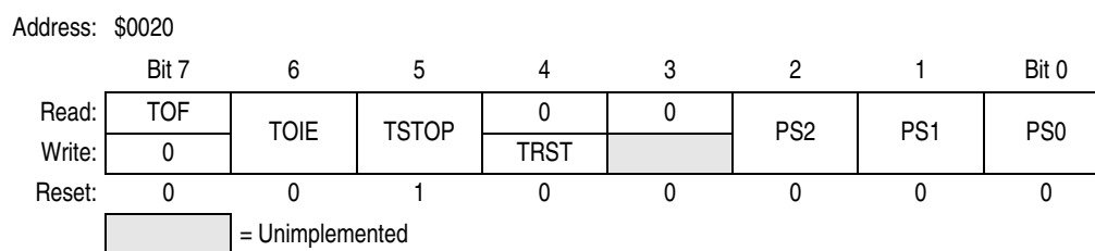
Figure 17-5. TIM1 Status and Control Register (T1SC)
