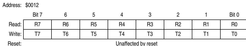
Figure 15-16. SPI Data Register (SPDR)
