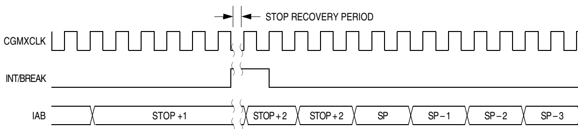
Figure 14-21. Stop Mode Recovery from Interrupt
