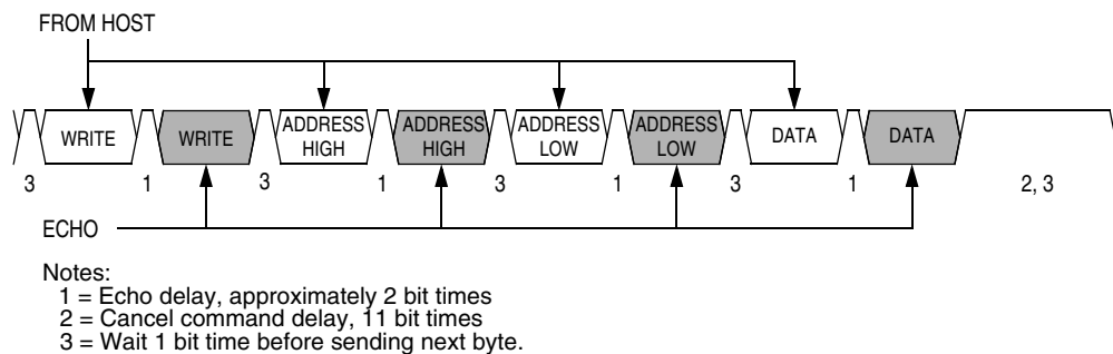
Figure 19-14. Write Transaction
