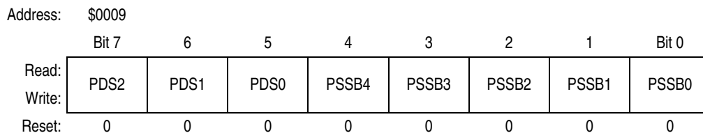
Figure 13-18. ESCI Prescaler Register (SCPSC)
