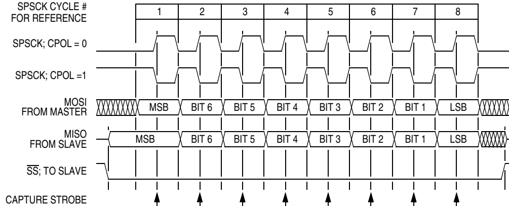
Figure 15-5. Transmission Format ( CPHA = 0 )
