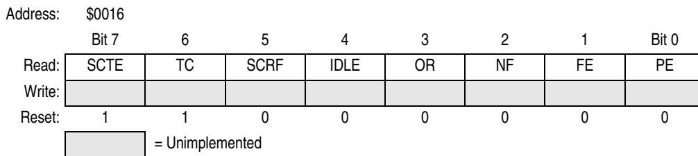
Figure 13-13. ESCI Status Register 1 (SCS1)
