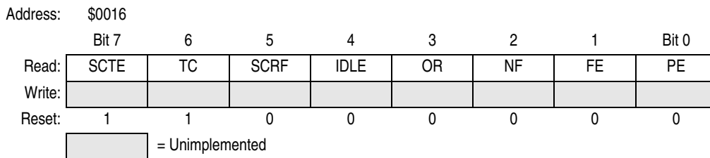
Figure 14-13. ESCI Status Register 1 (SCS1)
