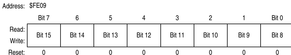
Figure 20-5. Break Address Register High (BRKH)
