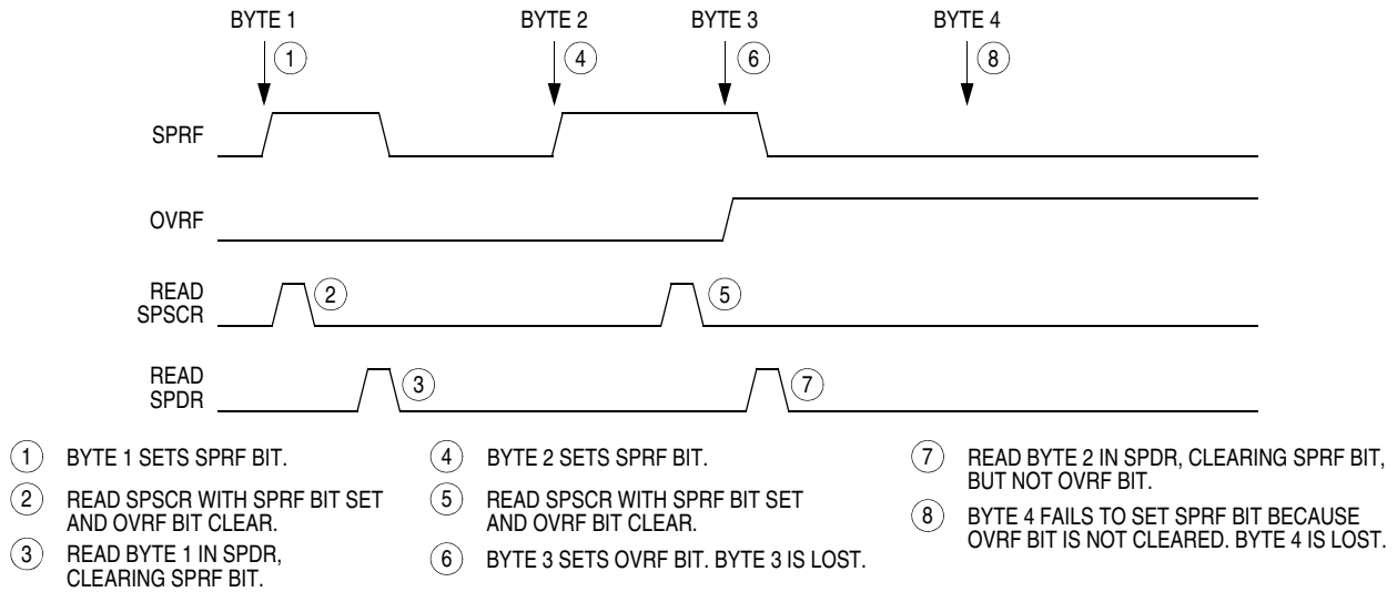
Figure 16-10. Missed Read of Overflow Condition
