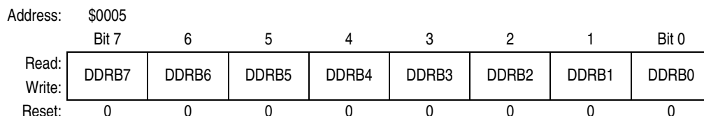
Figure 13-7. Data Direction Register B (DDRB)
