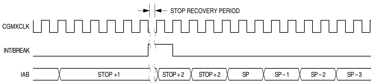
Figure 15-21. Stop Mode Recovery from Interrupt
