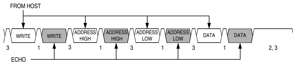
Figure 20-13. Read Transaction
