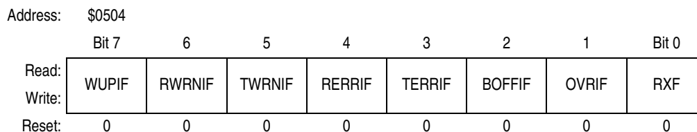
Figure 12-20. Receiver Flag Register (CRFLG)
