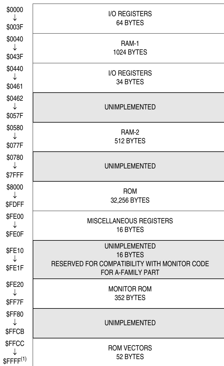
Figure 2-1. Memory Map
