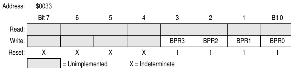
Figure 4-4. FLASH1 Block Protect Register (FL1BPR)
