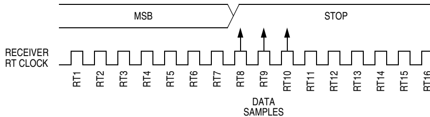
Figure 12-9. Slow Data
