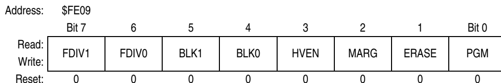
Figure 4-3. FLASH2 Control Register (FL2CR)
