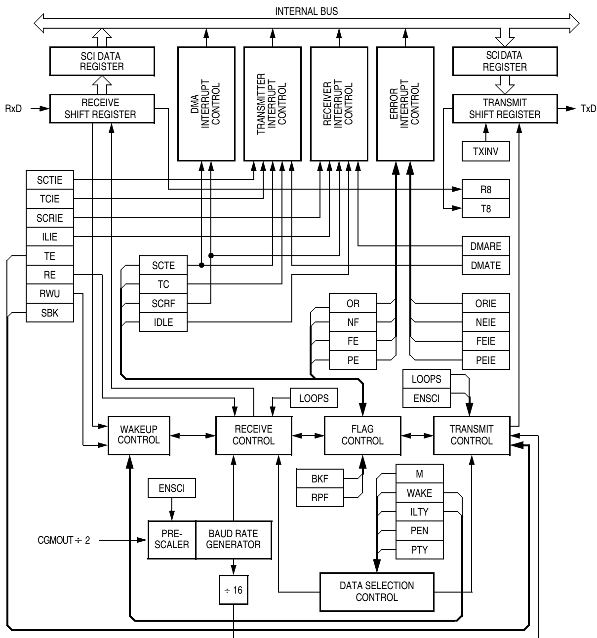
Figure 12-4. SCI Module Block Diagram
