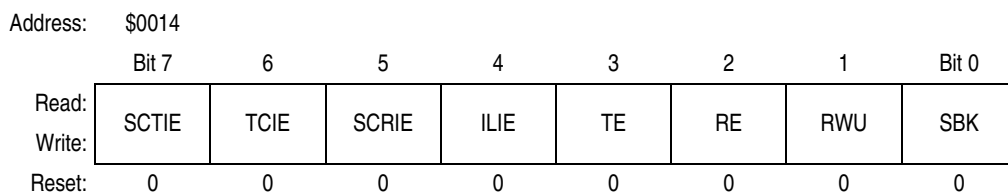
Figure 12-12. SCI Control Register 2 (SCC2)
