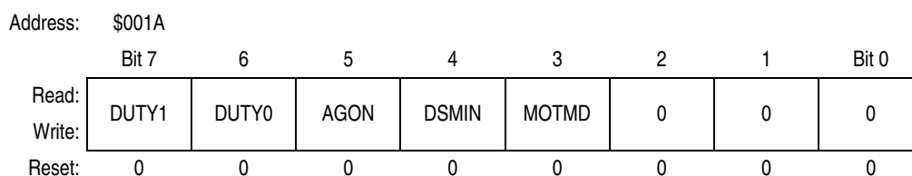
Figure 15-2. LCD Control Register (LCDCR)
