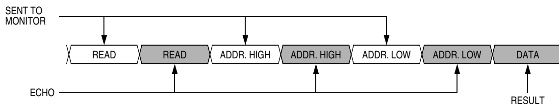
Figure 18-4. Read Transaction
