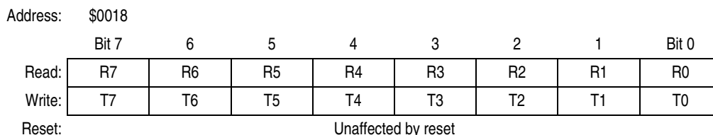
Figure 12-17. SCI Data Register (SCDR)
