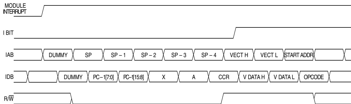
Figure 6-8. Interrupt Entry
