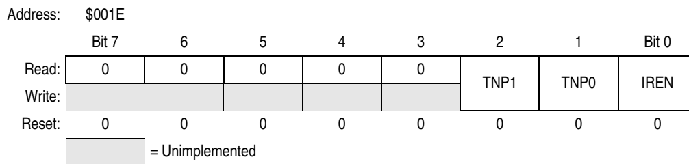
Figure 12-19. SCI Infrared Control Register (SCIRCR)
