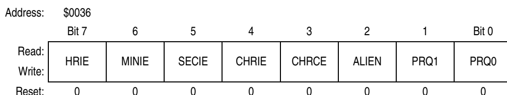
Figure 8-5. RTC Control Register (RTCCR)
