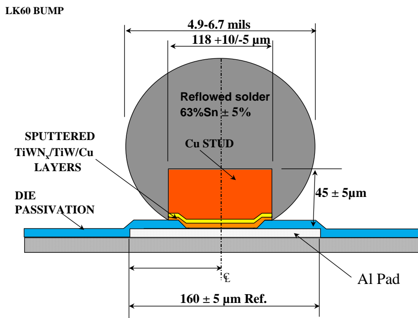
SMD Electroplated Bump : Dimensions Before Probe
