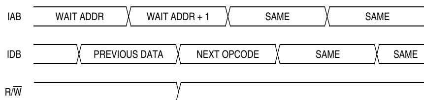
Figure 6-12. Wait Mode Entry Timing
