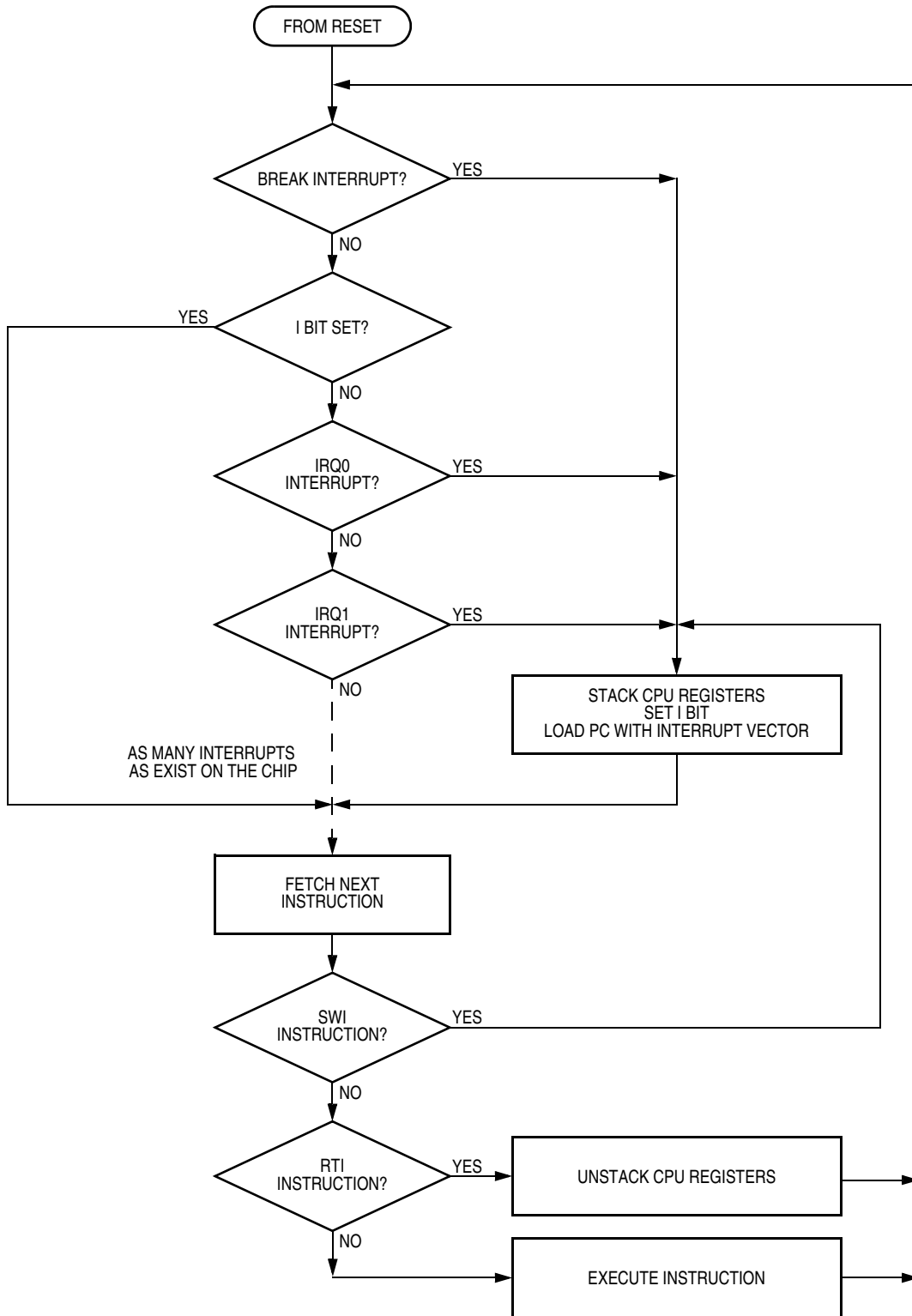
Figure 6-10. Interrupt Processing
