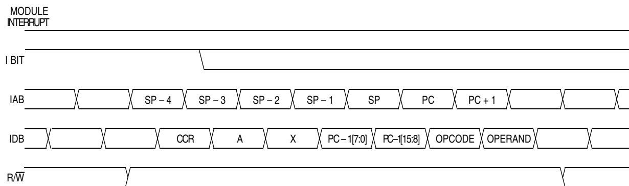
Figure 6-9. Interrupt Recovery
