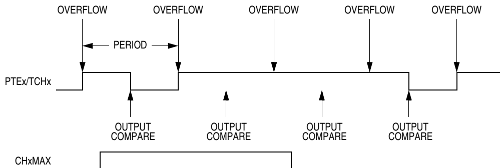
Figure 16-13. CHxMAX Latency
