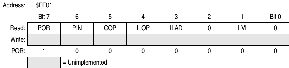
Figure 6-18. SIM Reset Status Register (SRSR)
