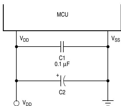
Figure 1-2. Power Supply Bypassing
