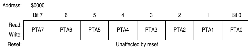
Figure 17-2. Port A Data Register (PTA)
