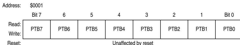
Figure 17-5. Port B Data Register (PTB)
