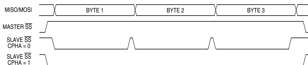
Figure 13-5. CPHA/SS Timing
