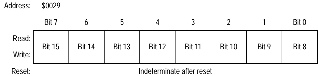
Figure 16-16. Timer Channel 1 Register High (TCH1H)
