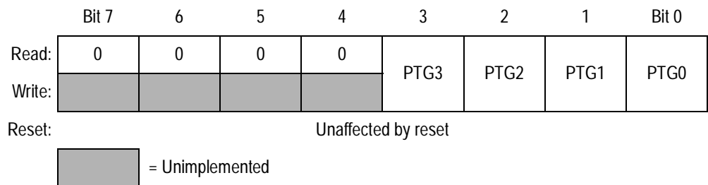
Figure 17-20. Port G Data Register (PTG)
