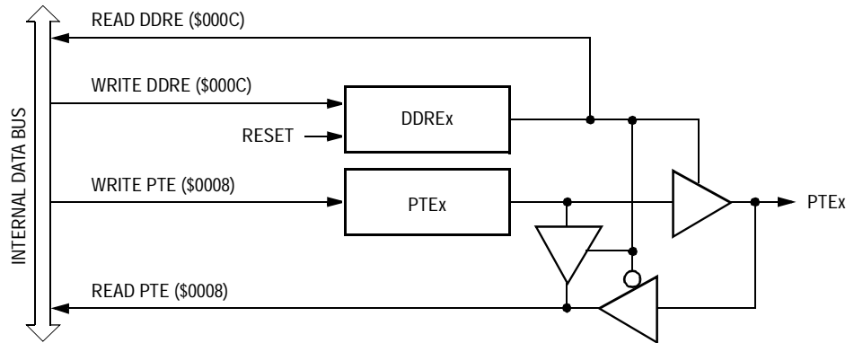
Figure 17-16. Port E I/O Circuit
