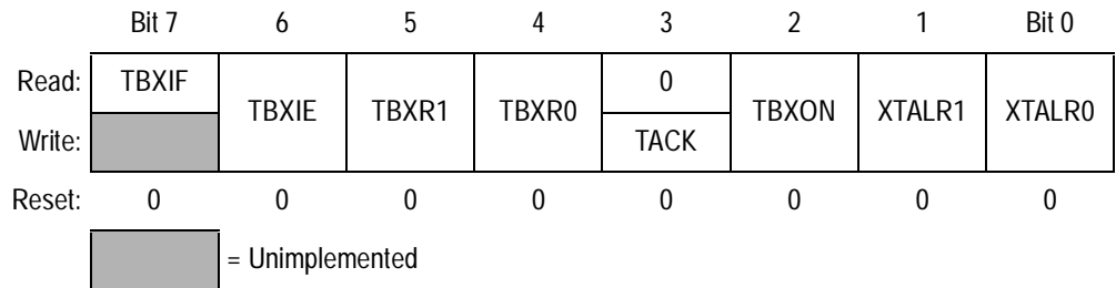
Figure 15-2. Timebase Control Register (TBXCR)
