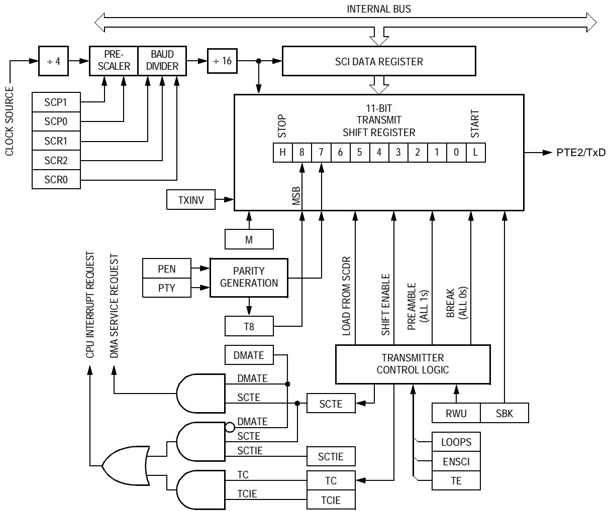
Figure 12-4. SCI Transmitter
