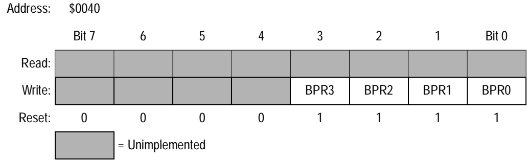
Figure 4-3. FLASH 1 Block Protect Register (FL1BPR)
