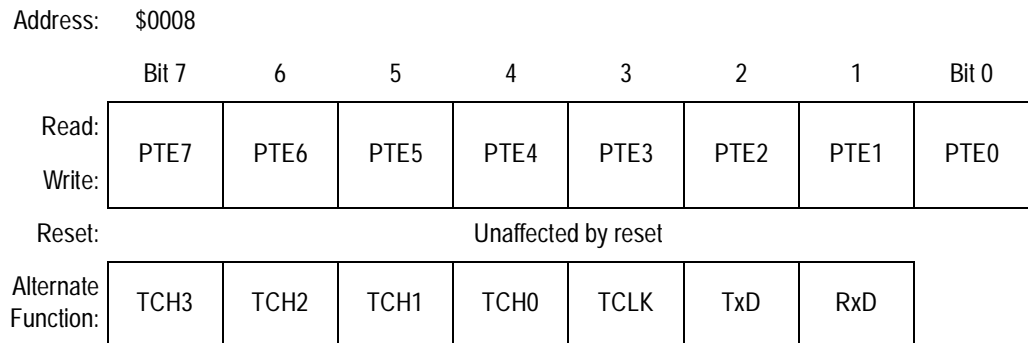
Figure 17-14. Port E Data Register (PTE)
