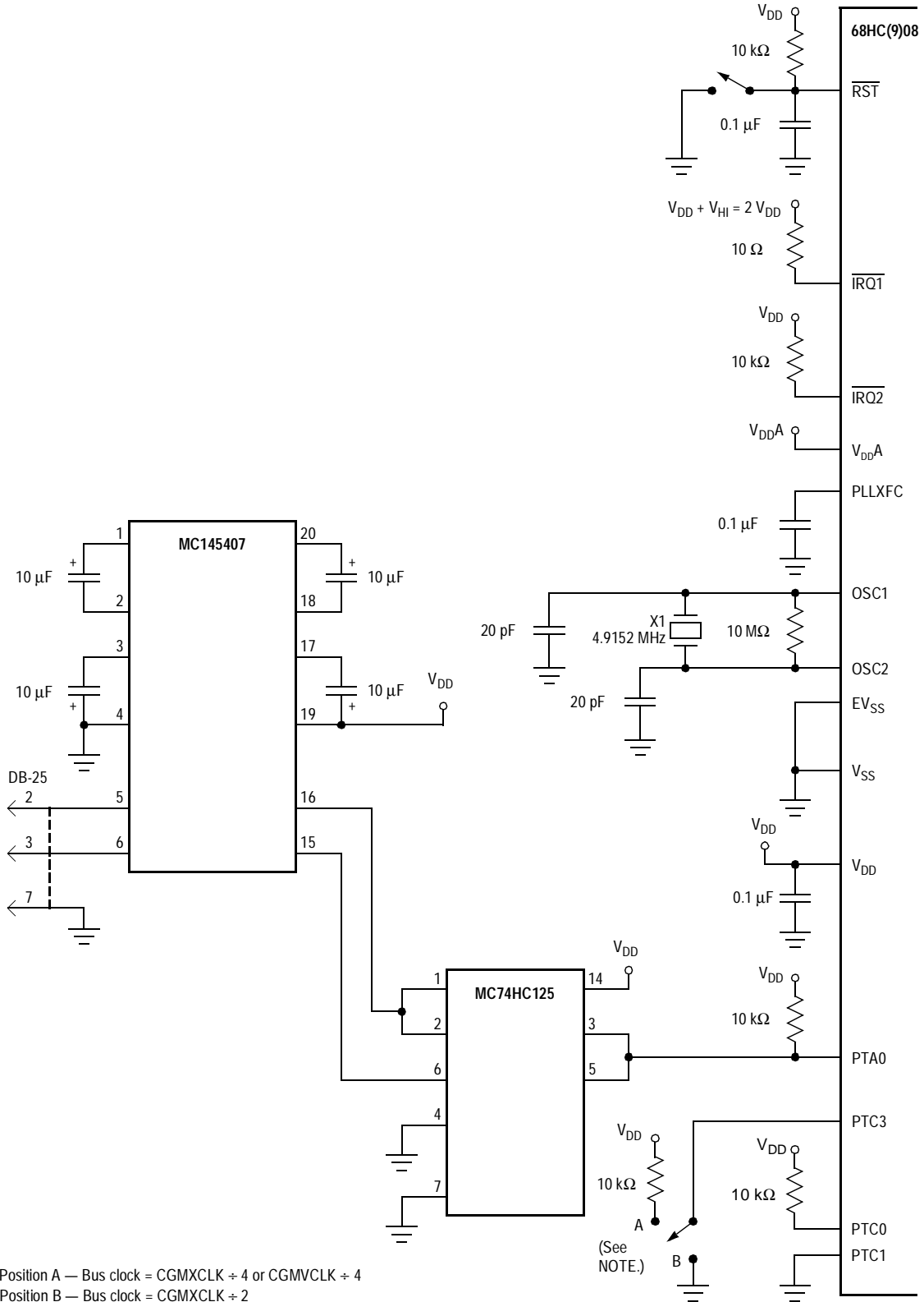
Figure 8-1. Monitor Mode Circuit
