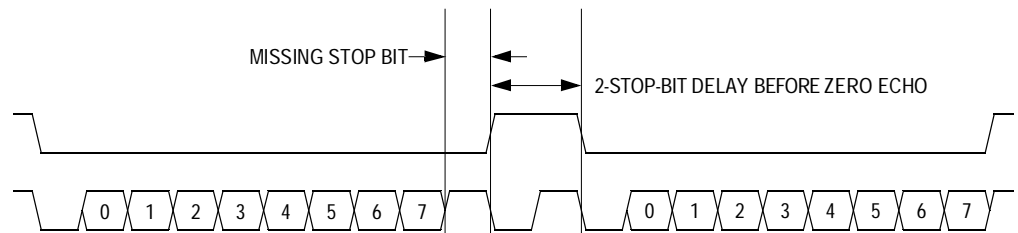
Figure 8-5. Break Transaction
