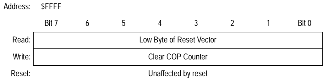
Figure 19-2. COP Control Register (COPCTL)
