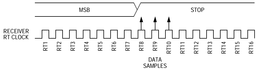
Figure 12-7. Slow Data
