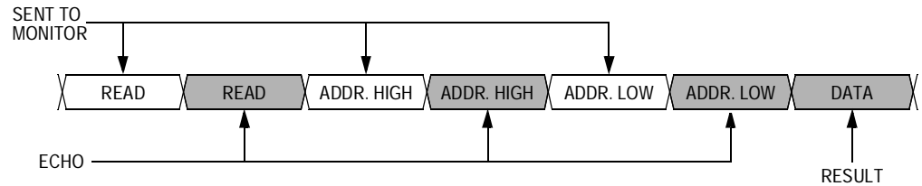
Figure 8-4. Read Transaction
