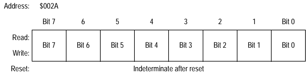
Figure 16-17. Timer Channel 1 Register Low (TCH1L)
