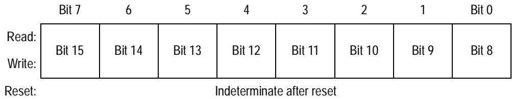
Figure 16-20. Timer Channel 3 Register High (TCH3H)
