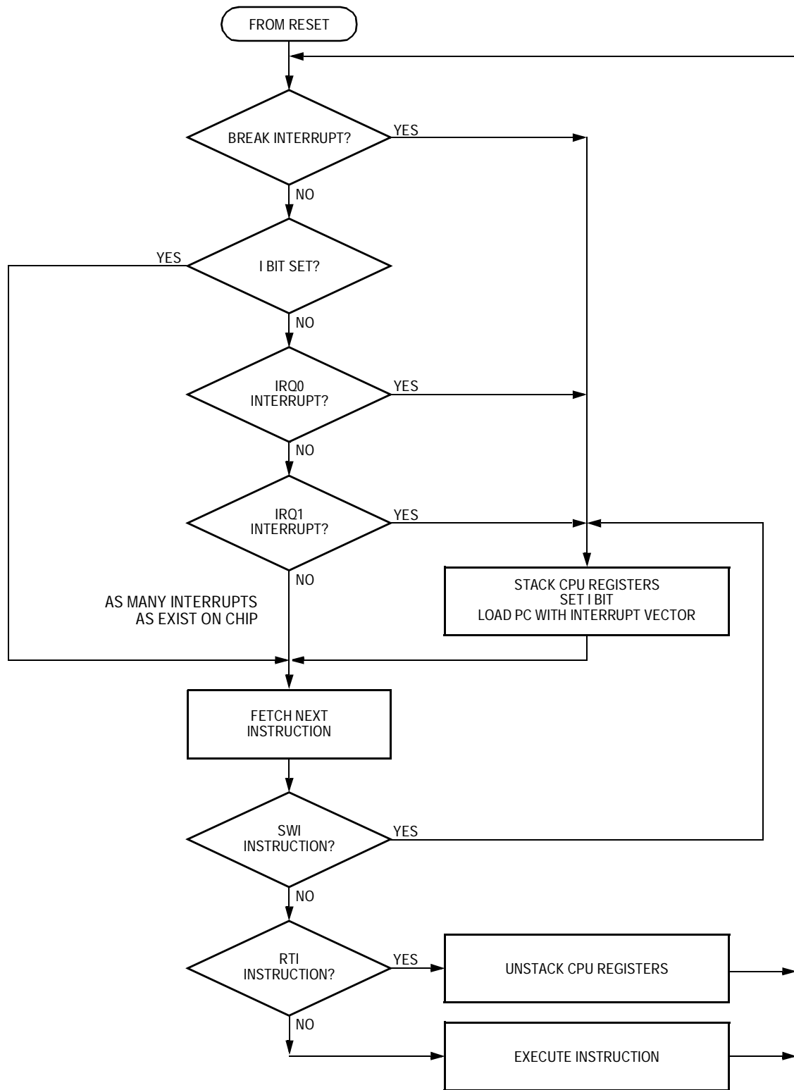
Figure 6-9. Interrupt Processing
