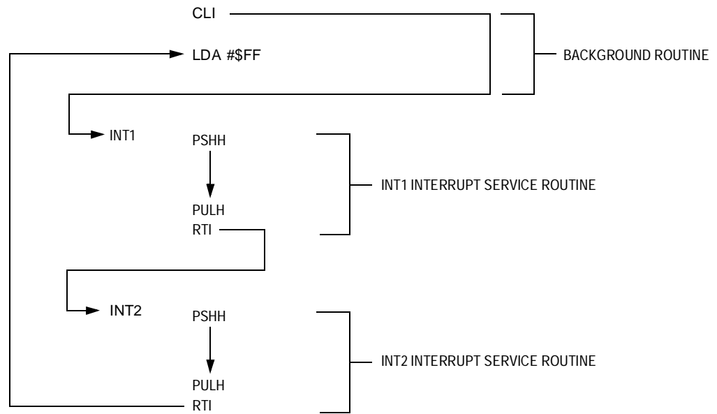
Figure 6-11. Interrupt Recognition Example
