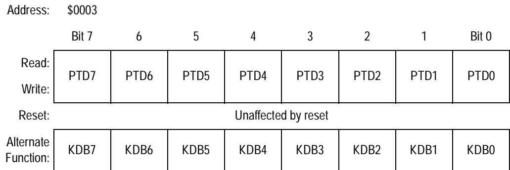
Figure 17-11. Port D Data Register (PTD)
