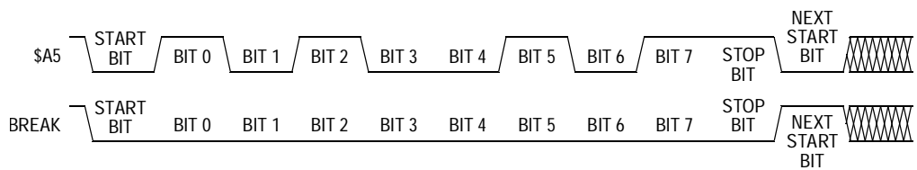
Figure 8-3. Sample Monitor Waveforms
