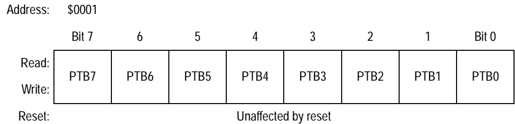
Figure 17-5. Port B Data Register (PTB)
