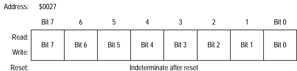
Figure 16-15. Timer Channel 0 Register Low (TCH0L)
