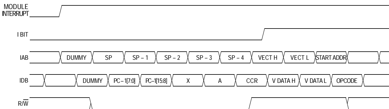
Figure 6-8. Interrupt Entry
