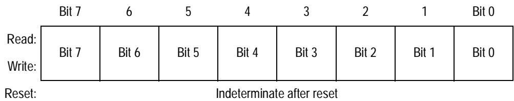
Figure 16-21. Timer Channel 3 Register Low (TCH3L)
