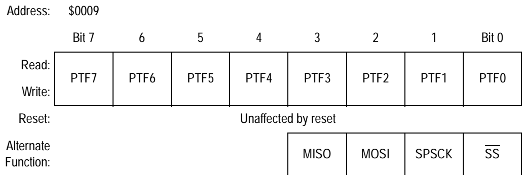
Figure 17-17. Port F Data Register (PTF)
