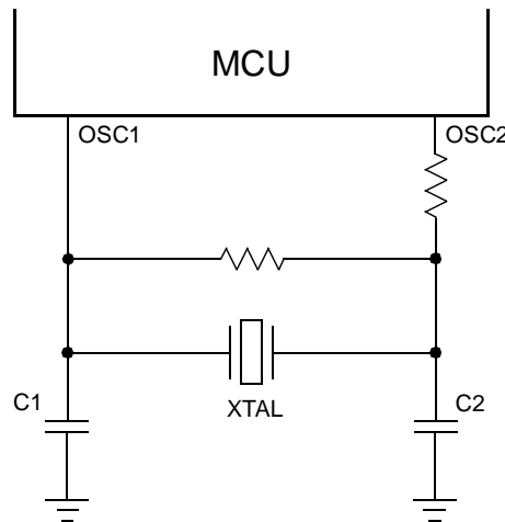
Figure 1-4. Crystal Connections
