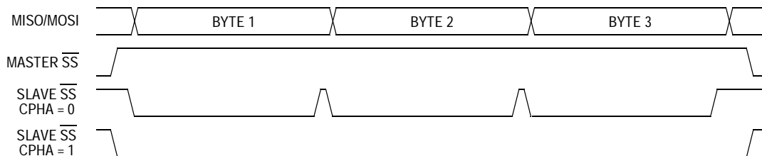
Figure 13-5. CPHA/ \overline{SS} Timing
