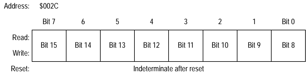
Figure 16-18. Timer Channel 2 Register High (TCH2H)
