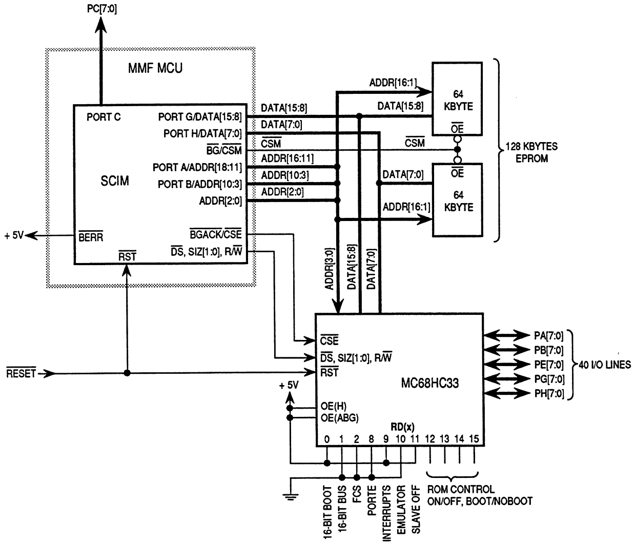
SCIM-PRU SINGLE CHIP EMUL SYS
