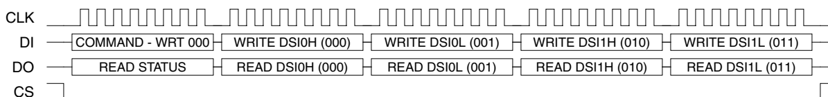
Figure 4-7. SPI Burst Transfer Example
