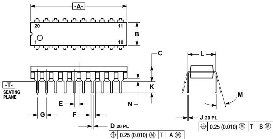
Figure 12-1. MC68HC705J2P (Case 738-03)
