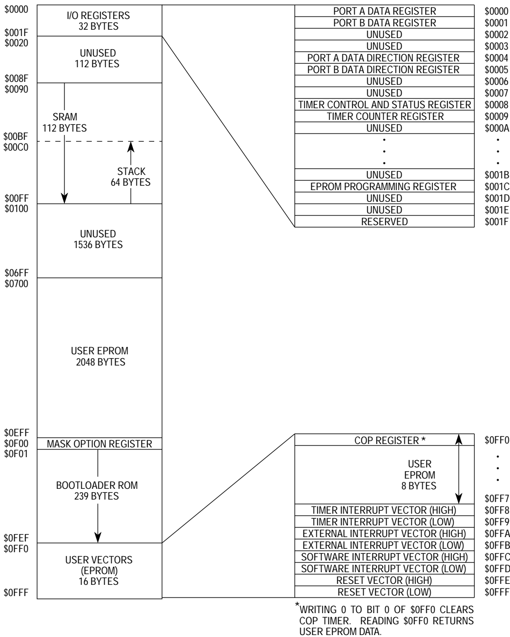
Figure 6-1. Memory Map
