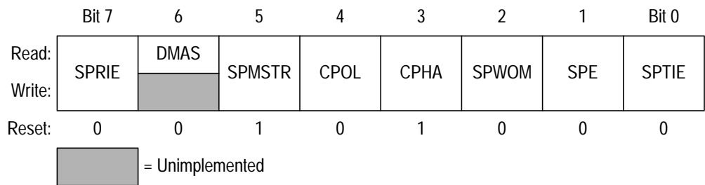
Figure 13-13. SPI Control Register (SPCR)
