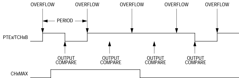
Figure 12-8. CHxMAX Latency
