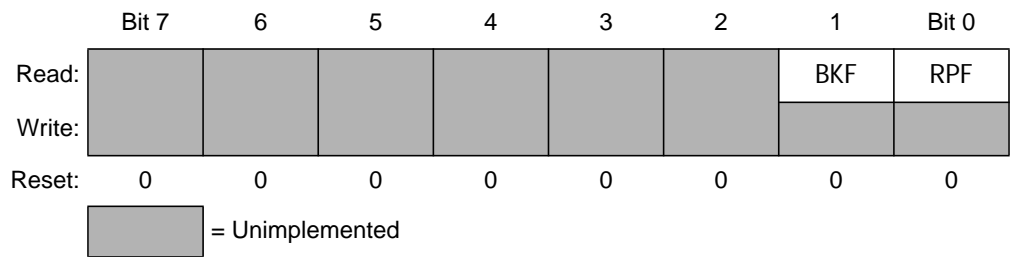
Figure 14-12. SCI Status Register 2 (SCS2)
