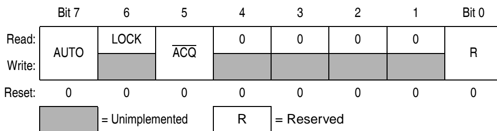
Figure 7-5. PLL Bandwidth Control Register (PBWC)
