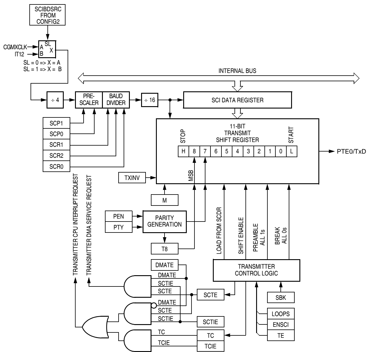
Figure 18-4. SCI Transmitter
