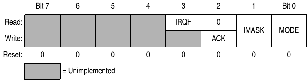
Figure 12-3. IRQ Status and Control Register (INTSCR)
