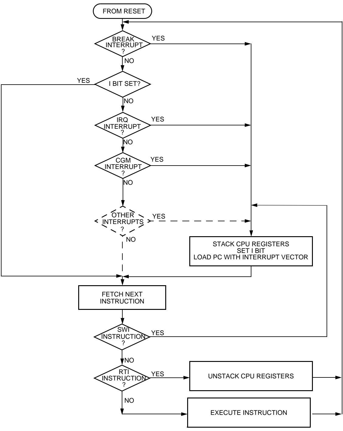
Figure 4-6. Interrupt Processing
