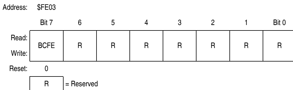
Figure 19-22. SIM Break Flag Control Register (SBFCR)
