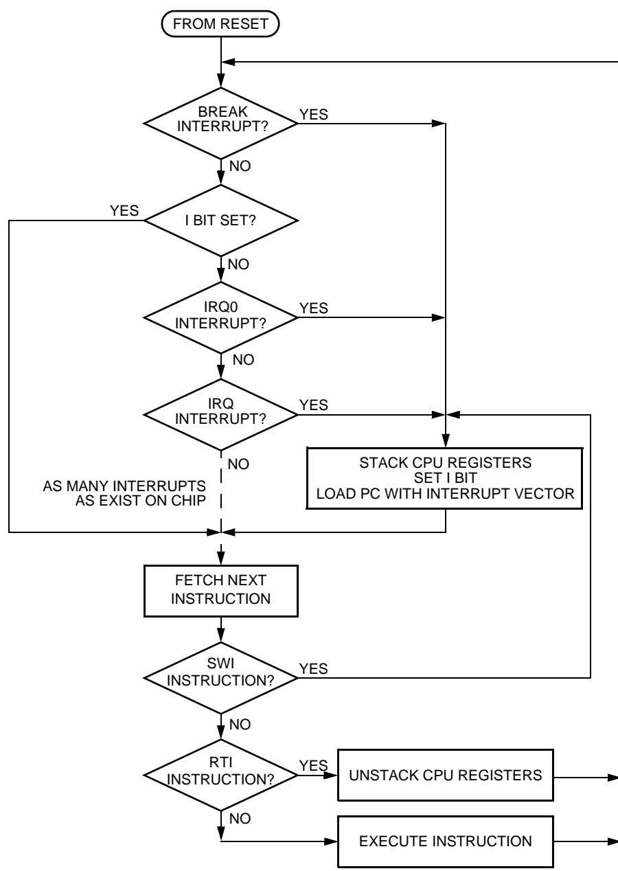
Figure 19-10. Interrupt Processing
