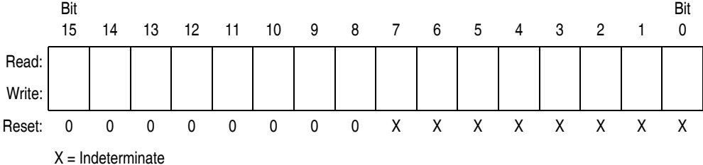
Figure 10-3. Index Register (H:X)
