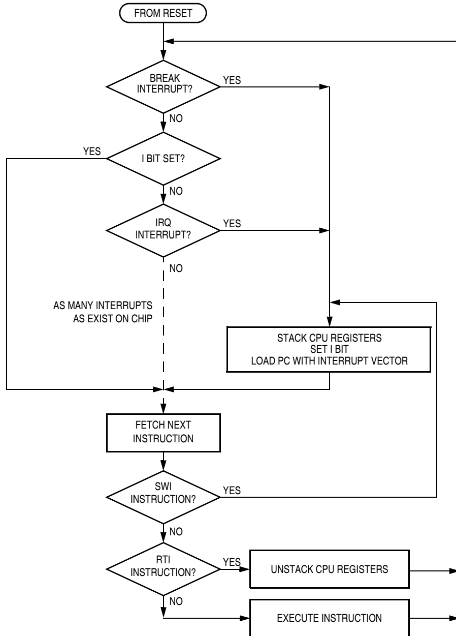
Figure 20-10. Interrupt Processing
