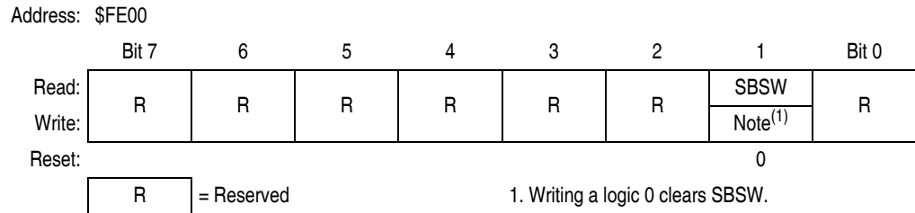
Figure 6-6. Break Status Register (BSR)
