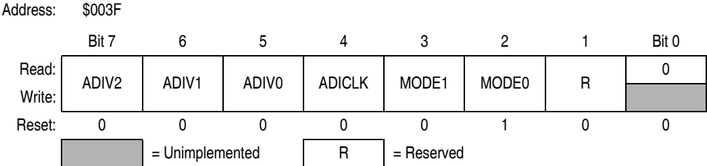
Figure 5-8. ADC Clock Register (ADCLK)
