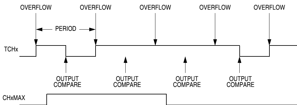
Figure 23-11. CHxMAX Latency
