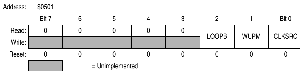
Figure 16-16. Module Control Register (CMCR1)
