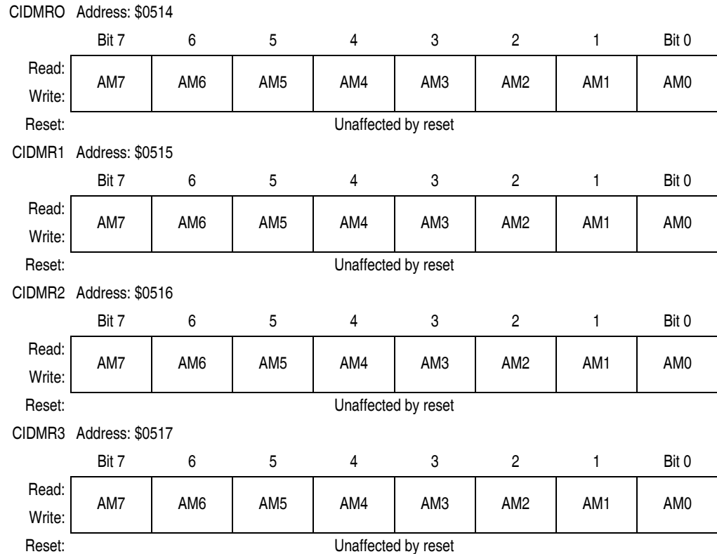
Figure 16-27. Identifier Mask Registers (CIDMR0–CIDMR3)
