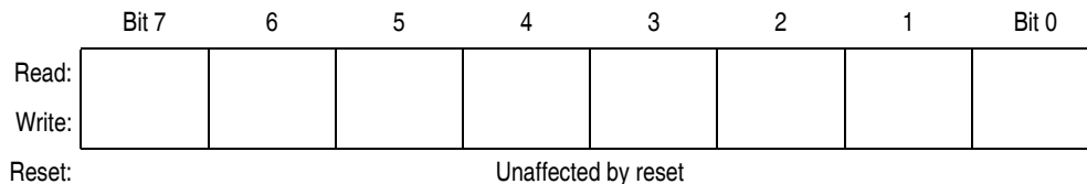
Figure 10-2. Accumulator (A)
