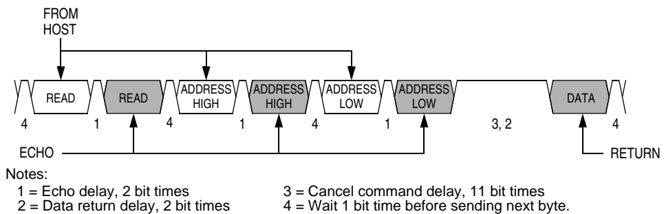
Figure 13-10. Read Transaction
