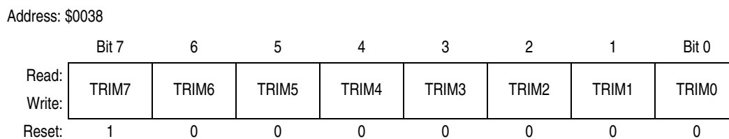
Figure 6-13. ICG Trim Register (ICGTR)
