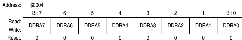
Figure 9-3. Data Direction Register A (DDRA)
