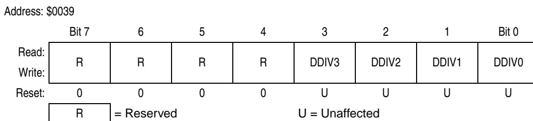
Figure 6-14. ICG DCO Divider Register (ICGDVR)
