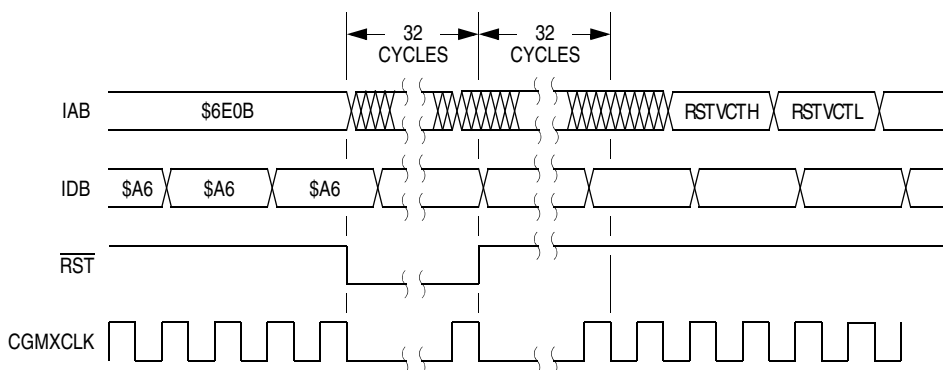
Figure 10-14. Wait Recovery from Internal Reset
