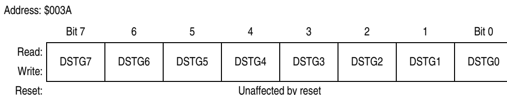
Figure 6-15. ICG DCO Stage Register (ICGDSR)
