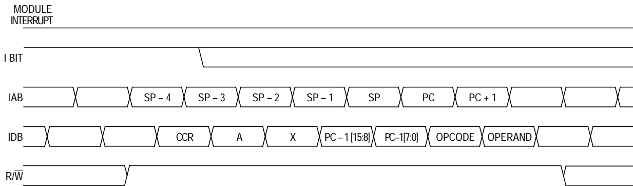
Figure 6-10. Interrupt Recovery
