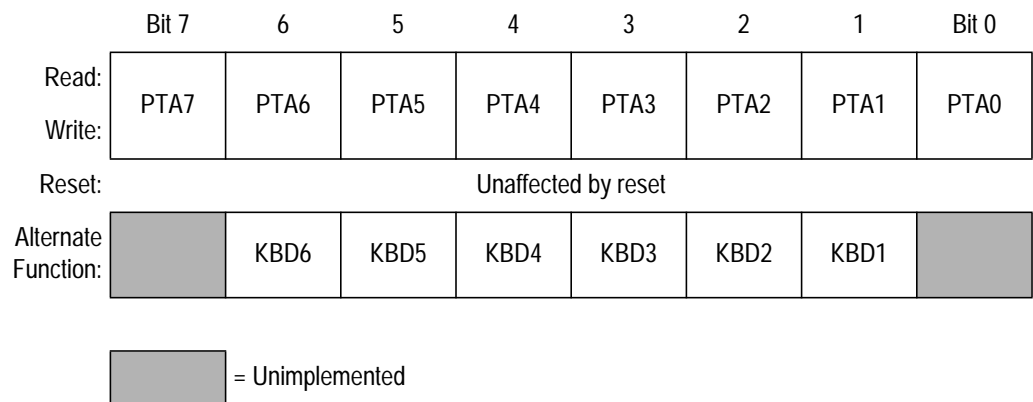
Figure 13-2. Port A Data Register (PTA)
