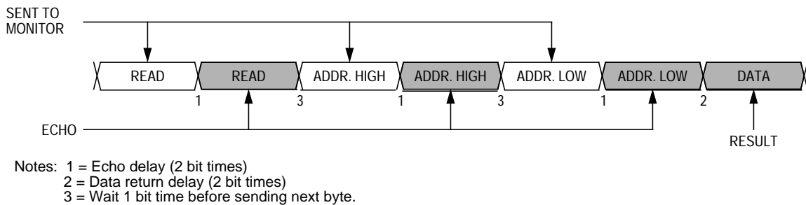
Figure 10-4. Read Transaction
