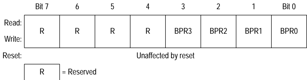
Figure 4-3. FLASH 2TS Block Protect Register (FLBPR)
