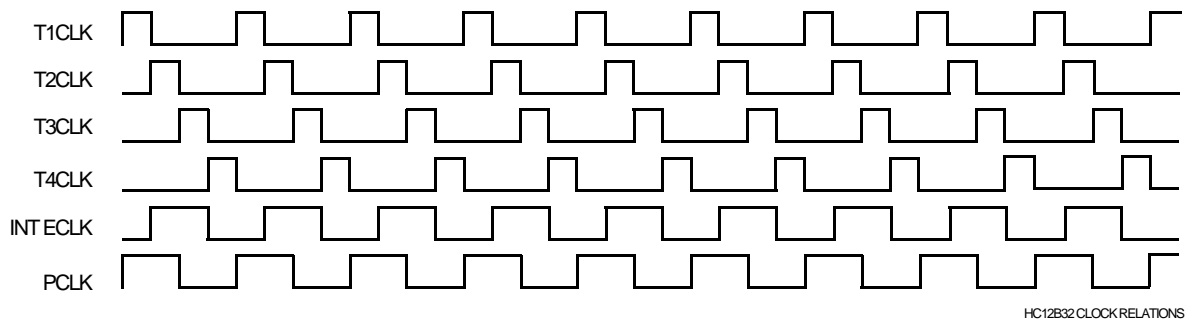
Figure 12 Internal Clock Relationships
