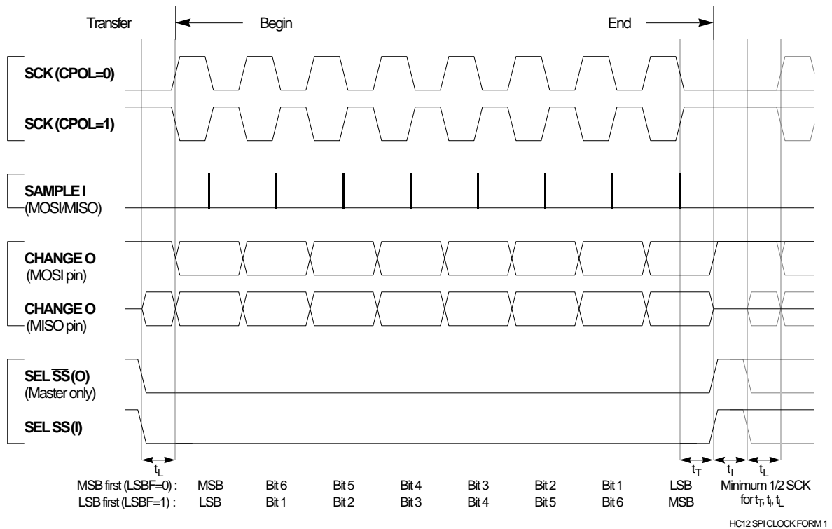
Figure 25 SPI Clock Format 1 (CPHA = 1)
