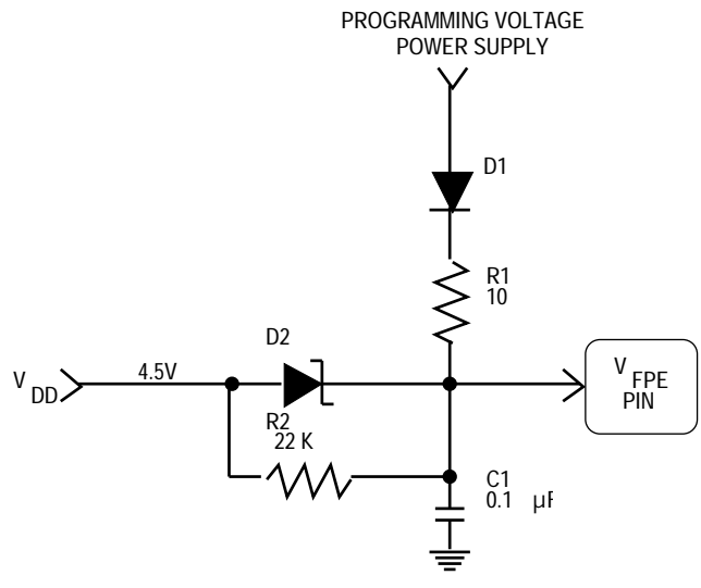
Figure 10 V FPE Conditioning Circui
