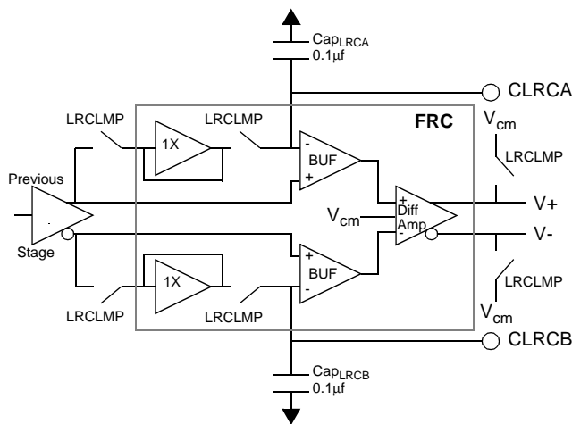
Figure 13. FRC Conceptual Block Diagram
