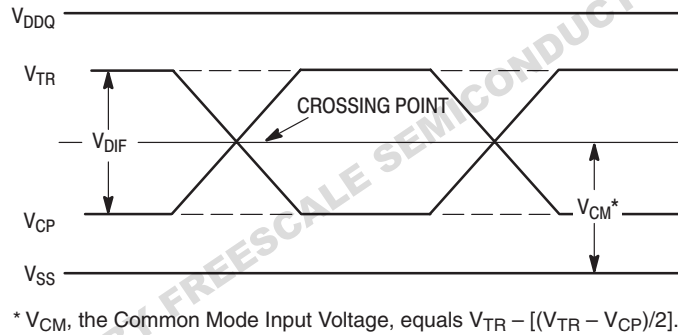
Figure 2. Differential Inputs/Common Mode Input Voltage
