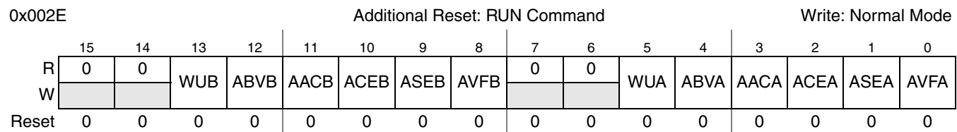
Figure 3-21. Protocol Status Register 3 (PSR3)
