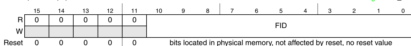
Figure 3-95. Message Buffer Frame ID Registers (MBFIDRn)
