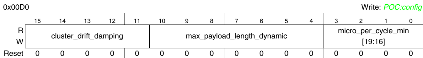
Figure 3-86. Protocol Configuration Register 24 (PCR24)
