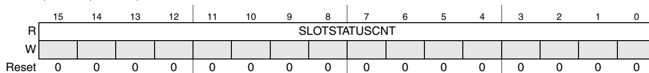
Figure 3-45. Slow Status Counter Registers (SSCR0–SSCR3)
