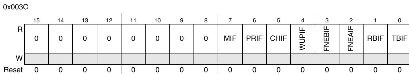
Figure 3-28. Combined Interrupt Flag Register (CIFRR)
