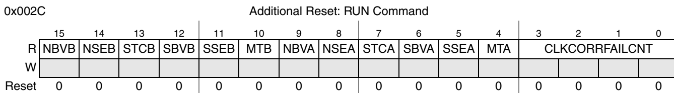
Figure 3-20. Protocol Status Register 2 (PSR2)
