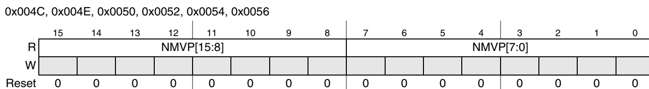
Figure 3-35. Network Management Vector Registers (NMVR0–NMVR5)
