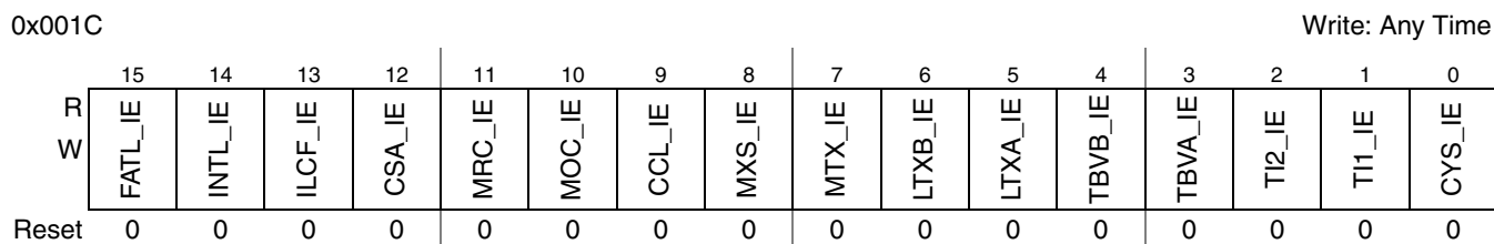
Figure 3-12. Protocol Interrupt Enable Register 0 (PIER0)
