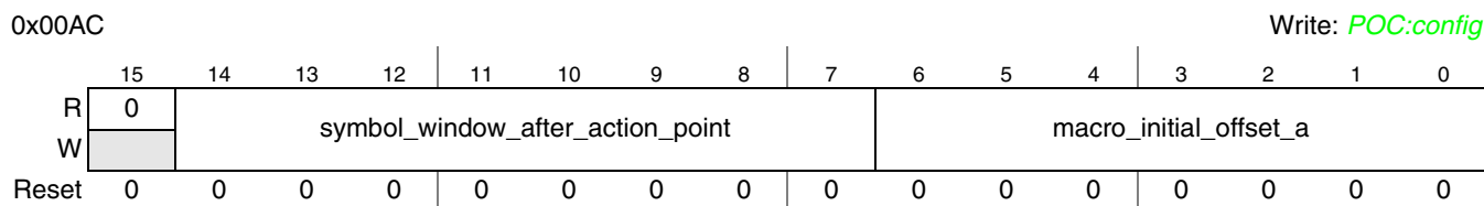
Figure 3-68. Protocol Configuration Register 6 (PCR6)
