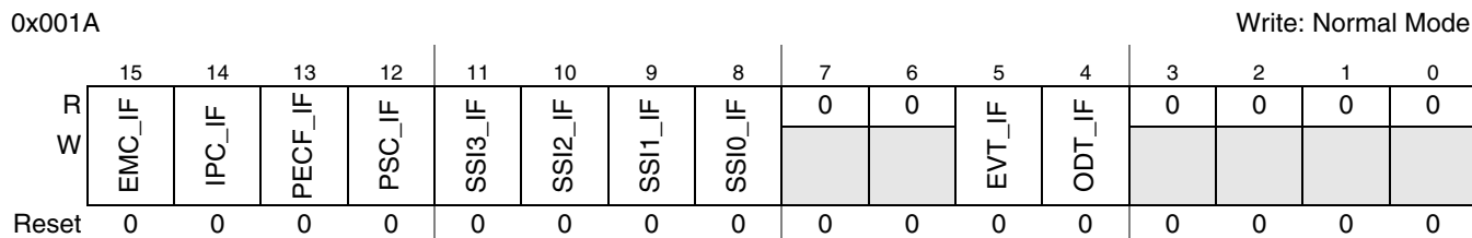
Figure 3-11. Protocol Interrupt Flag Register 1 (PIFR1)
