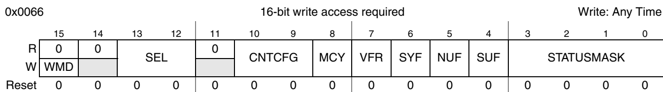
Figure 3-43. Slot Status Counter Condition Register (SSCCR)
