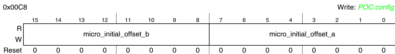
Figure 3-82. Protocol Configuration Register 20 (PCR20)
