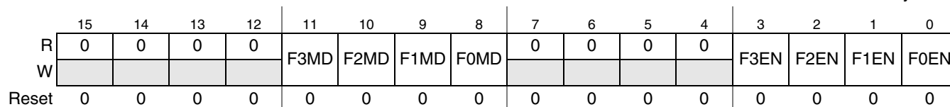
Figure 3-59. Receive FIFO Range Filter Control Register (RFRFCTR)
