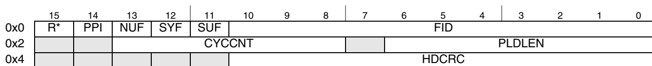
Figure 3-102. Frame Header Structure
