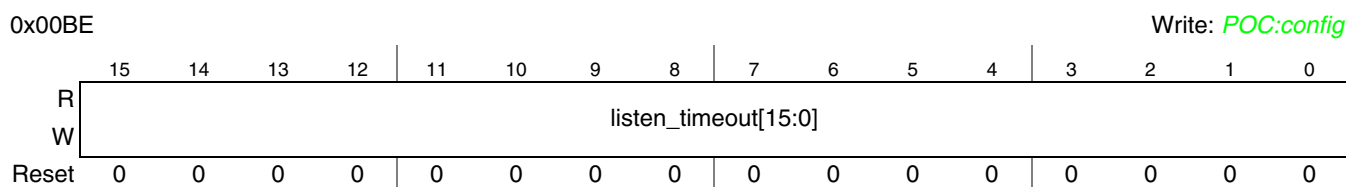
Figure 3-77. Protocol Configuration Register 15 (PCR15)
