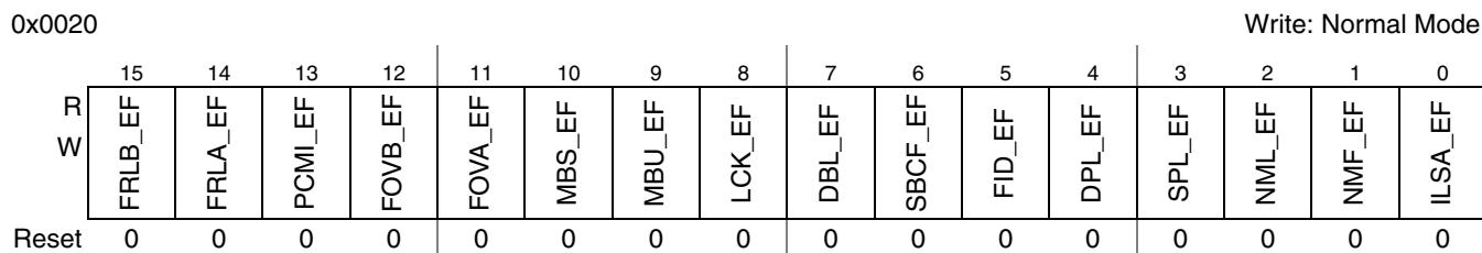
Figure 3-14. CHI Error Flag Register (CHIERFR)
