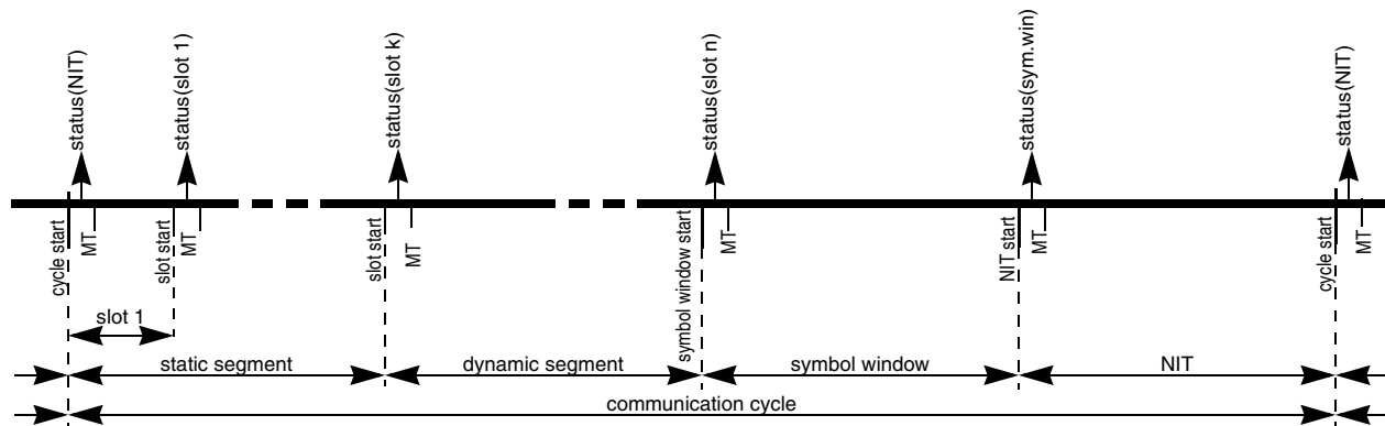
Figure 3-139. Slot Status Vector Update
