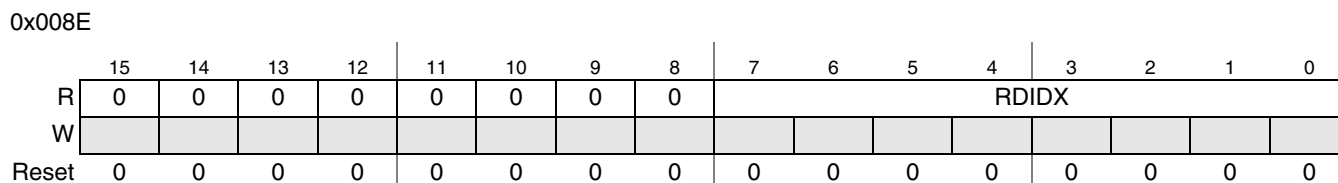
Figure 3-53. Receive FIFO B Read Index Register (RFBRIR)
