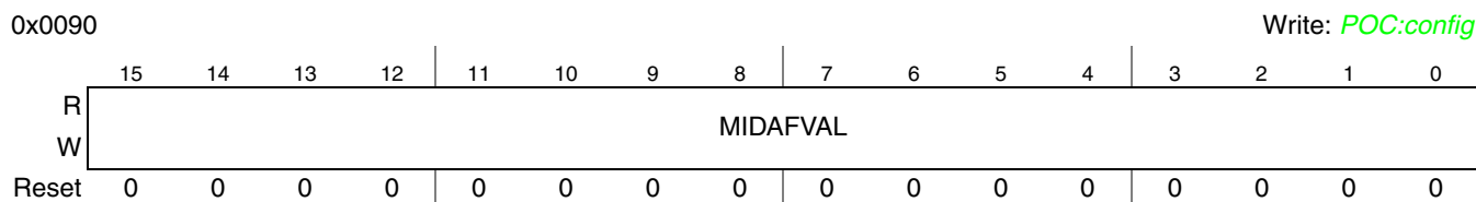
Figure 3-54. Receive FIFO Message ID Acceptance Filter Value Register (RFMIDAFVR)
