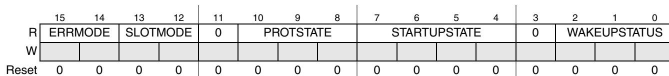
Figure 3-18. Protocol Status Register 0 (PSR0)
