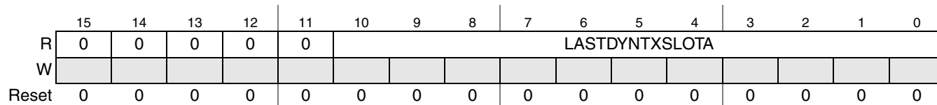
Figure 3-60. Last Dynamic Slot Channel A Register (LDTXSLAR)
