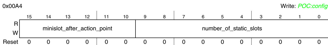
Figure 3-64. Protocol Configuration Register 2 (PCR2)
