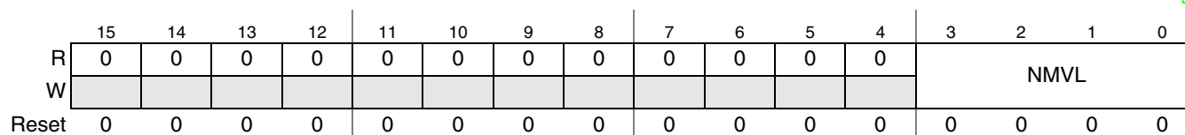
Figure 3-36. Network Management Vector Length Register (NMVLR)
