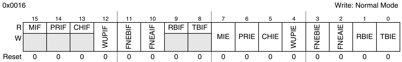
Figure 3-9. Global Interrupt Flag and Enable Register (GIFER)
