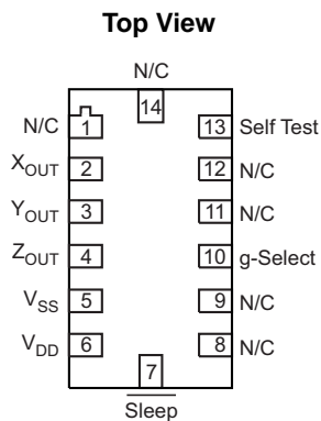
Figure 4. Pinout Description
