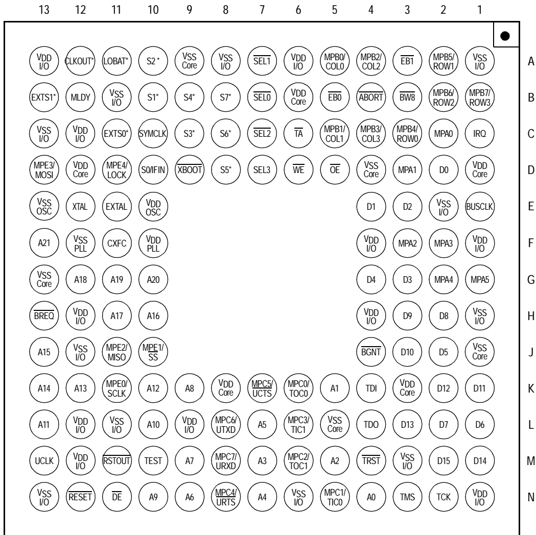
Figure 4. MMC2080/2075 BGA (144-Pin) Bottom View
