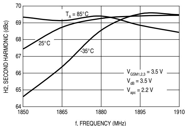
Figure 13. Second Harmonic Output versus Frequency
