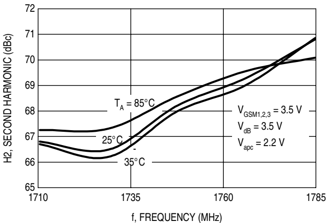
Figure 9. Second Harmonic Output versus Frequency
