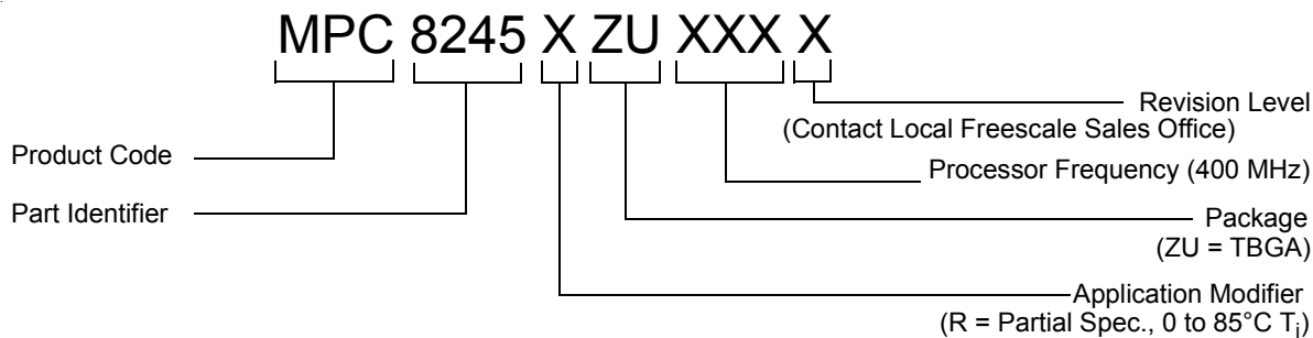
Figure 33. Freescale Part Number Key
