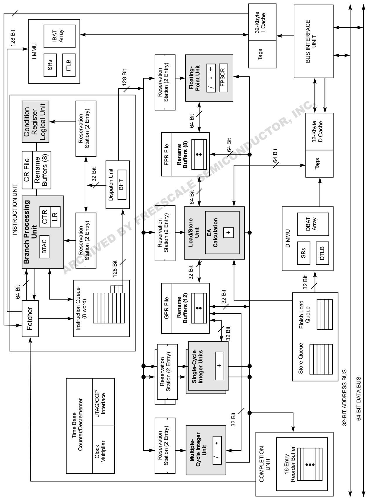
Figure 1. Block Diagram
