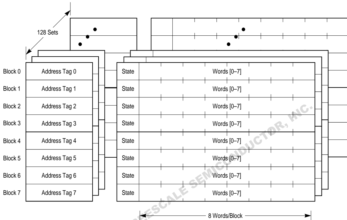
Figure 2. Cache Organization
