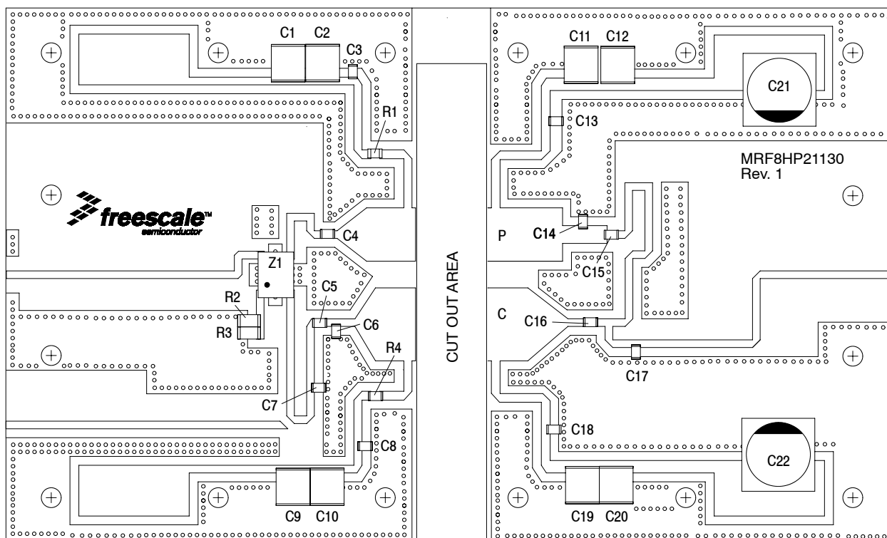
Figure 2. MRF8HP21130HR3(HSR3) Test Circuit Component Layout
