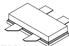
CASE 465H-02, STYLE 1 NI-780S-4 MRF8HP21130HSR3
