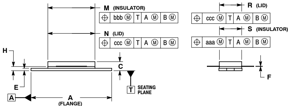
CASE 465-06 ISSUE G NI-780 MRF9135LR3
