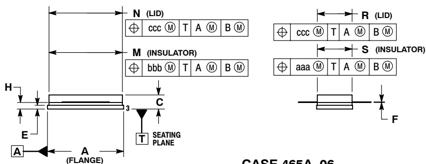
CASE 465A-06 ISSUE H NI-780S MRF9135LSR3
