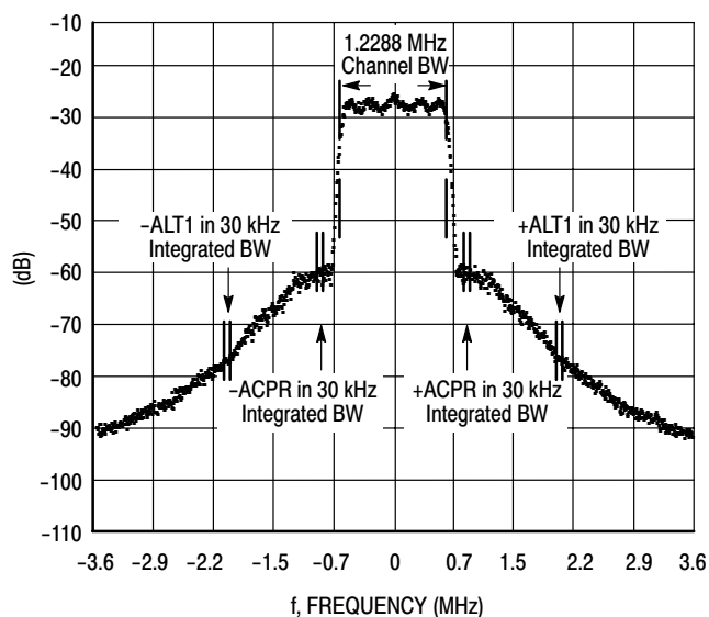
Figure 12. Single-Carrier N-CDMA Spectrum
