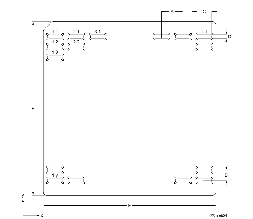
Fig 56. Tray details
