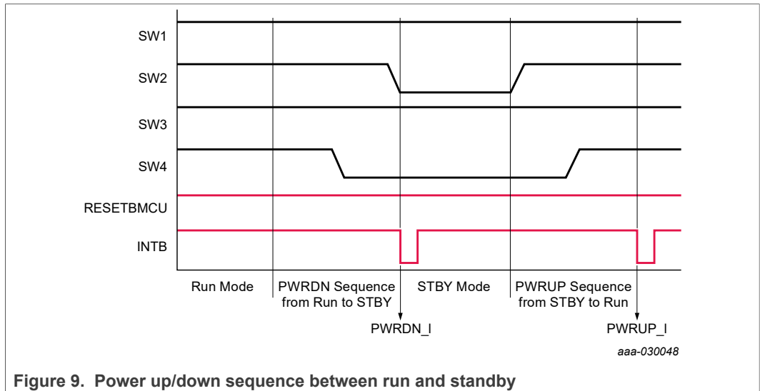
Figure 9. Power up/down sequence between run and standby
