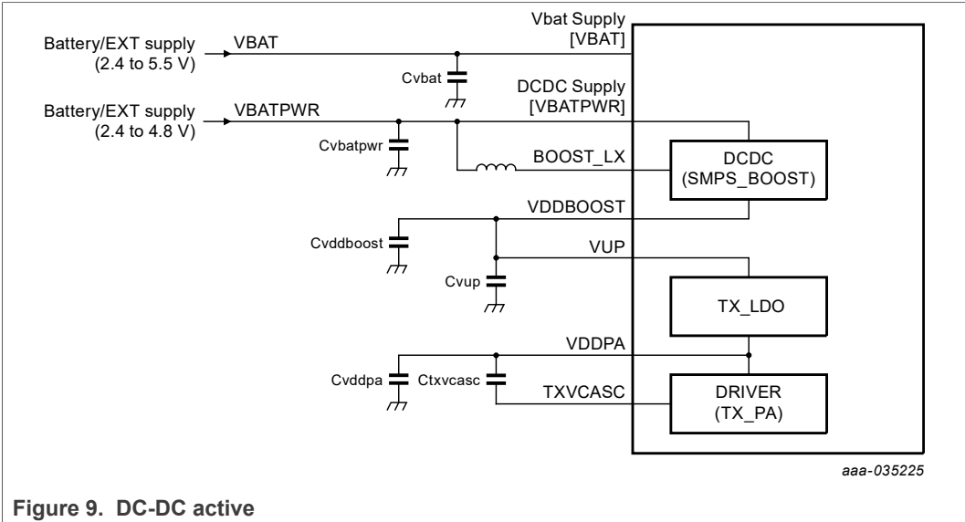
Figure 9. DC-DC active
