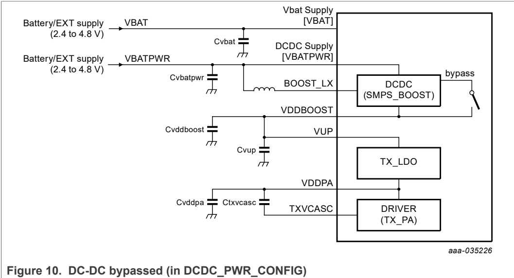
Figure 10. DC-DC bypassed (in DCDC_PWR_CONFIG)
