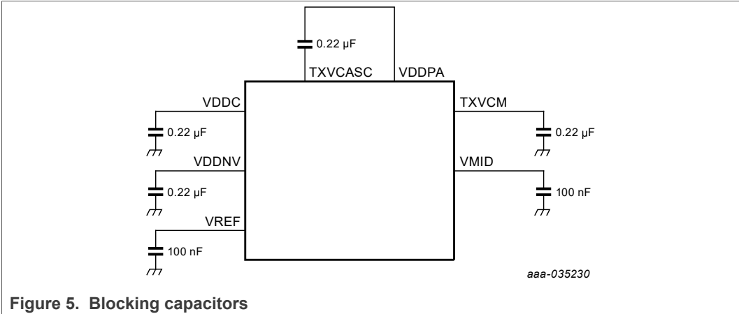
Figure 5. Blocking capacitors
