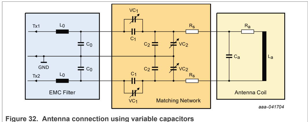
Figure 32. Antenna connection using variable capacitors
