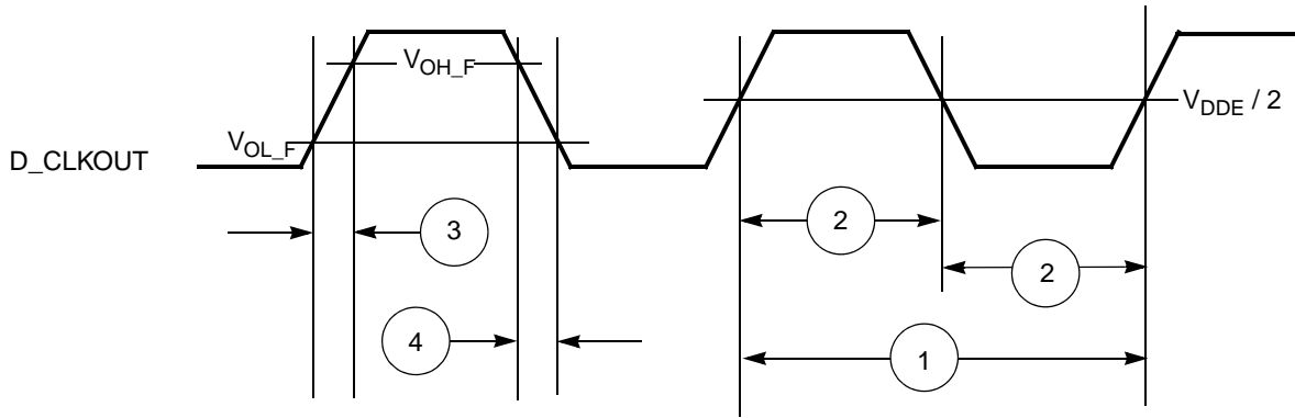
Figure 55. D_CLKOUT timing
